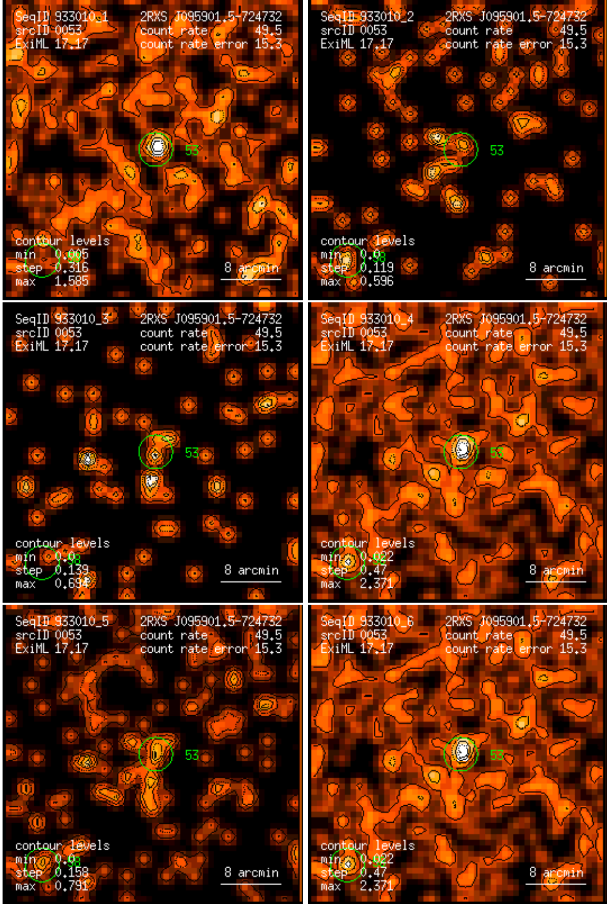
Figure 53: RASS 933010: detection 0053: band rate images, Gaussian filter: (1) PSPC channels 11 – 41, (2) 52 – 90, (3) 91 – 201, (4) 11 – 235, (5) 52 – 201, (6) 11 – 201. Broad band rates in counts/ks. Band rate contour levels in counts/ks/arcmin 2 .
