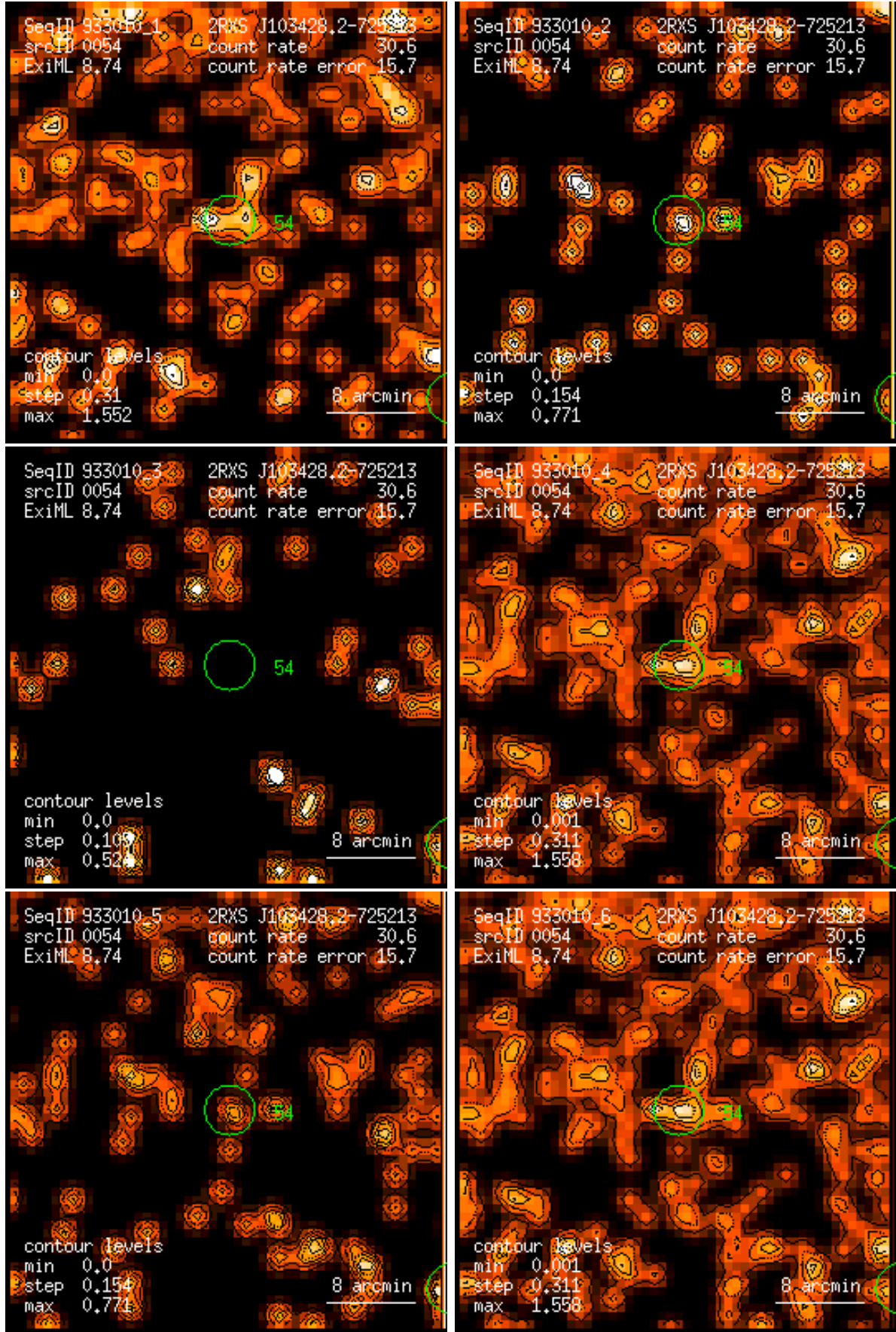
Figure 54: RASS 933010: detection 0054: band rate images, Gaussian filter: (1) PSPC channels 11 – 41, (2) 52 – 90, (3) 91 – 201, (4) 11 – 235, (5) 52 – 201, (6) 11 – 201. Broad band rates in counts/ks. Band rate contour levels in counts/ks/arcmin 2 .
