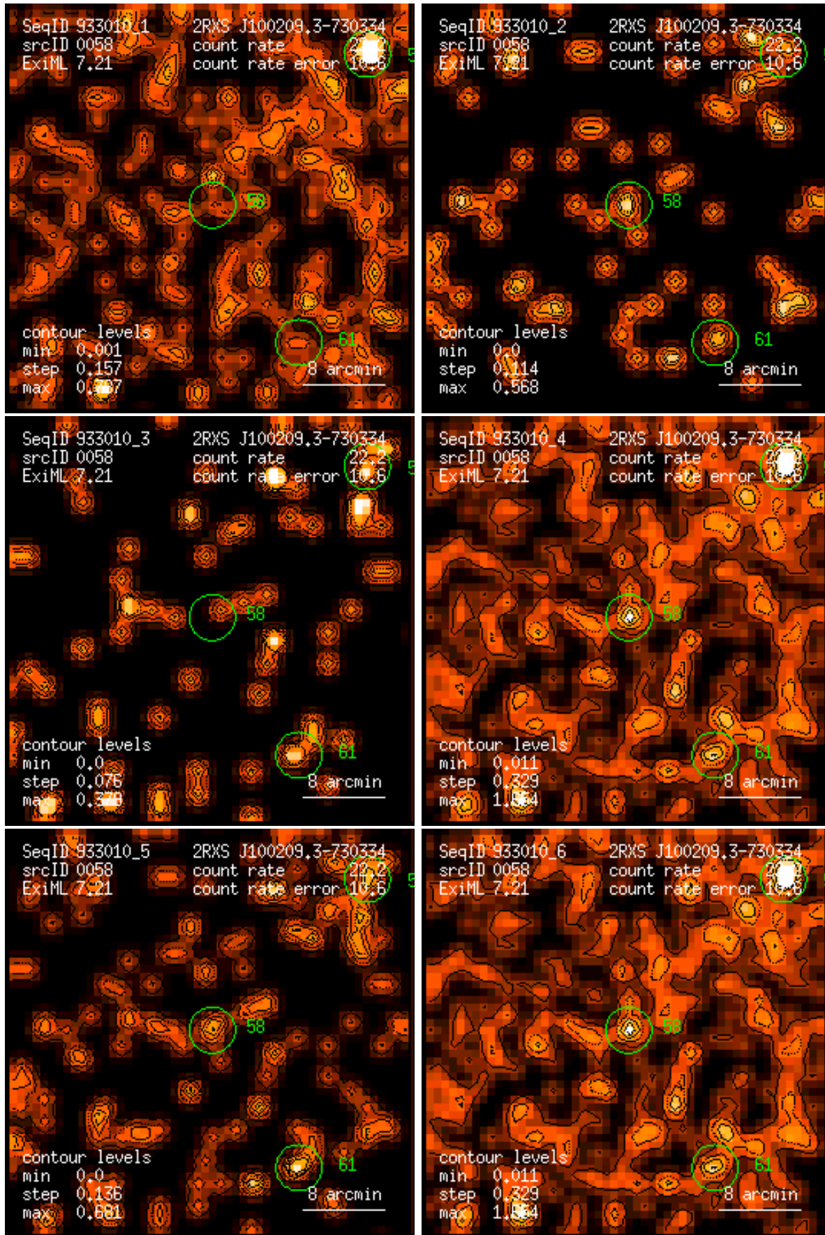
Figure 58: RASS 933010: detection 0058: band rate images, Gaussian filter: (1) PSPC channels 11 – 41, (2) 52 – 90, (3) 91 – 201, (4) 11 – 235, (5) 52 – 201, (6) 11 – 201. Broad band rates in counts/ks. Band rate contour levels in counts/ks/arcmin 2 .
