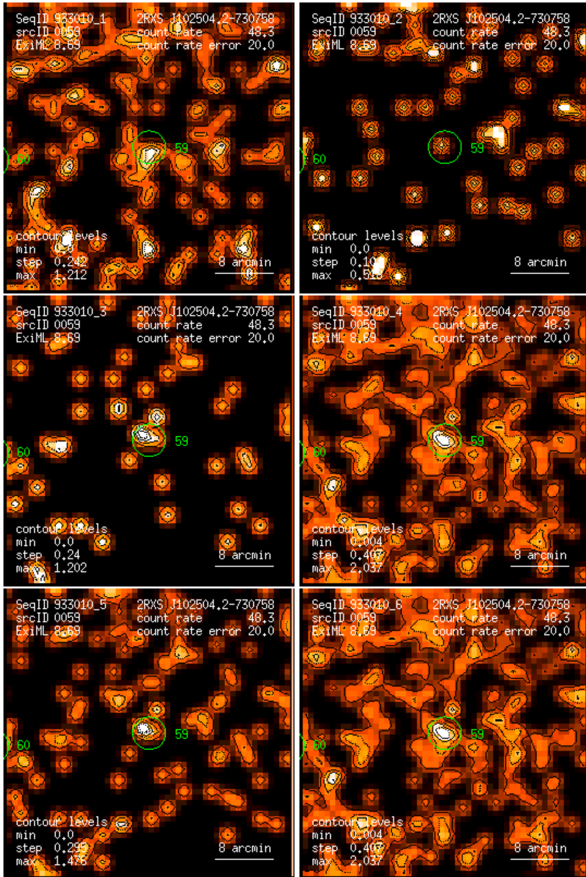
Figure 59: RASS 933010: detection 0059: band rate images, Gaussian filter: (1) PSPC channels 11 – 41, (2) 52 – 90, (3) 91 – 201, (4) 11 – 235, (5) 52 – 201, (6) 11 – 201. Broad band rates in counts/ks. Band rate contour levels in counts/ks/arcmin 2 .
