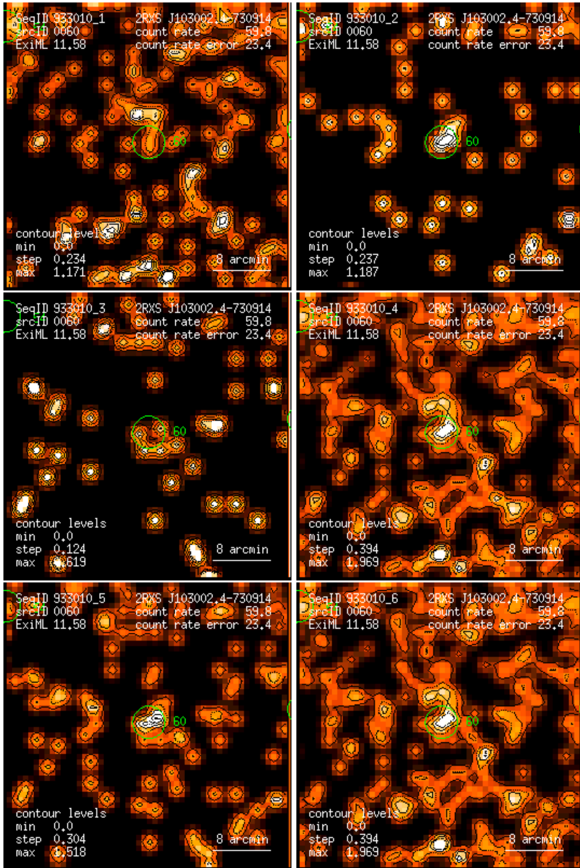
Figure 60: RASS 933010: detection 0060: band rate images, Gaussian filter: (1) PSPC channels 11 – 41, (2) 52 – 90, (3) 91 – 201, (4) 11 – 235, (5) 52 – 201, (6) 11 – 201. Broad band rates in counts/ks. Band rate contour levels in counts/ks/arcmin 2 .
