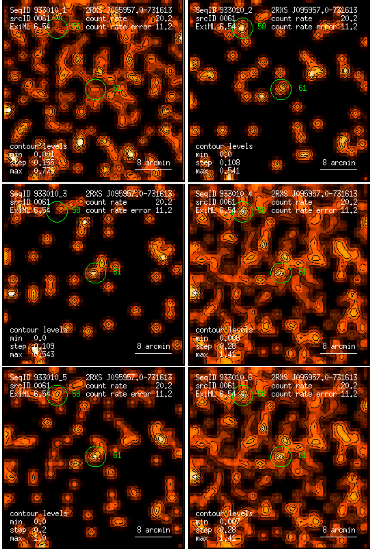
Figure 61: RASS 933010: detection 0061: band rate images, Gaussian filter: (1) PSPC channels 11 – 41, (2) 52 – 90, (3) 91 – 201, (4) 11 – 235, (5) 52 – 201, (6) 11 – 201. Broad band rates in counts/ks. Band rate contour levels in counts/ks/arcmin 2 .
