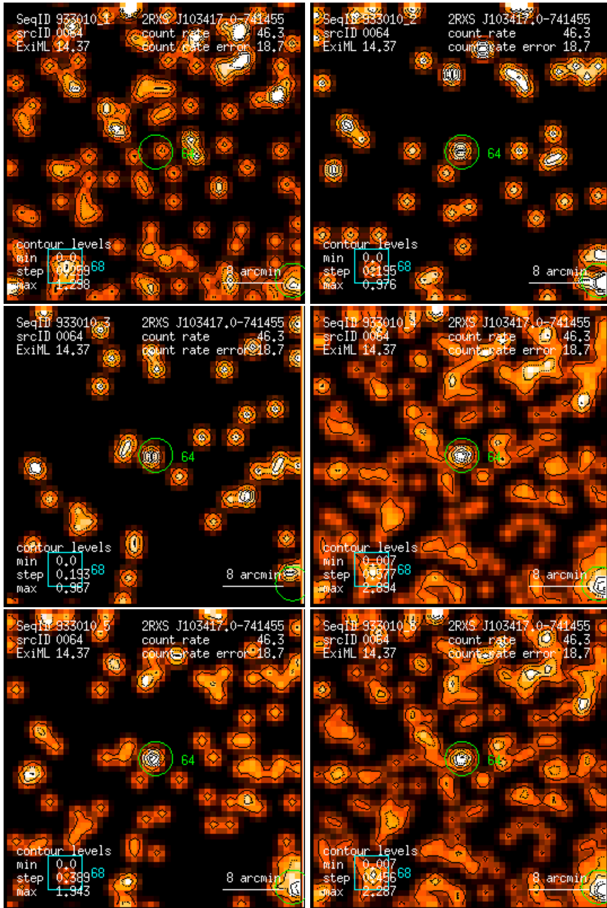
Figure 64: RASS 933010: detection 0064: band rate images, Gaussian filter: (1) PSPC channels 11 – 41, (2) 52 – 90, (3) 91 – 201, (4) 11 – 235, (5) 52 – 201, (6) 11 – 201. Broad band rates in counts/ks. Band rate contour levels in counts/ks/arcmin 2 .
