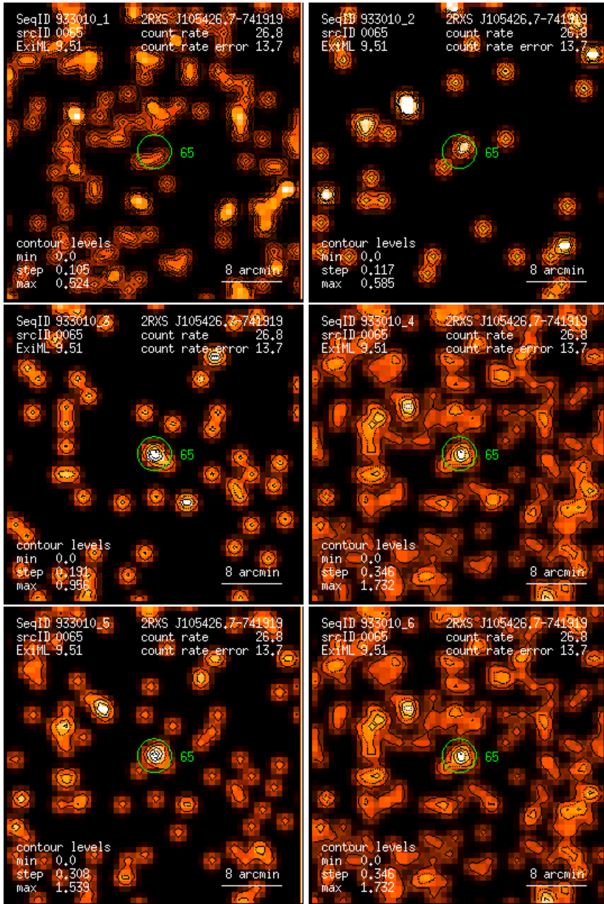
Figure 65: RASS 933010: detection 0065: band rate images, Gaussian filter: (1) PSPC channels 11 – 41, (2) 52 – 90, (3) 91 – 201, (4) 11 – 235, (5) 52 – 201, (6) 11 – 201. Broad band rates in counts/ks. Band rate contour levels in counts/ks/arcmin 2 .
