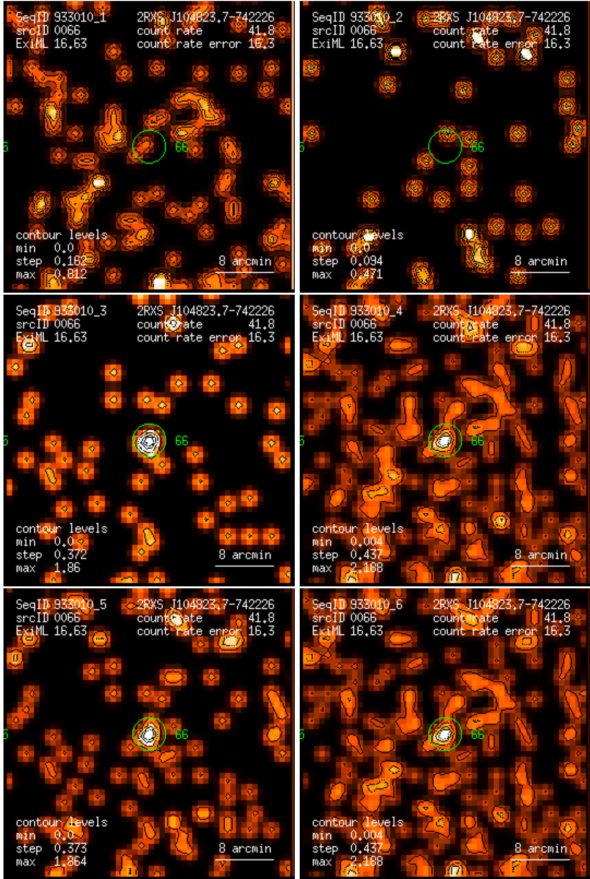
Figure 66: RASS 933010: detection 0066: band rate images, Gaussian filter: (1) PSPC channels 11 – 41, (2) 52 – 90, (3) 91 – 201, (4) 11 – 235, (5) 52 – 201, (6) 11 – 201. Broad band rates in counts/ks. Band rate contour levels in counts/ks/arcmin 2 .
