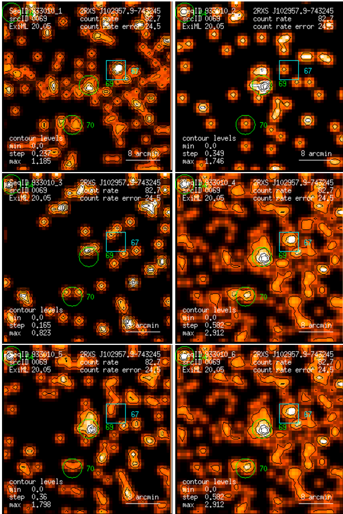
Figure 69: RASS 933010: detection 0069: band rate images, Gaussian filter: (1) PSPC channels 11 – 41, (2) 52 – 90, (3) 91 – 201, (4) 11 – 235, (5) 52 – 201, (6) 11 – 201. Broad band rates in counts/ks. Band rate contour levels in counts/ks/arcmin 2 .
