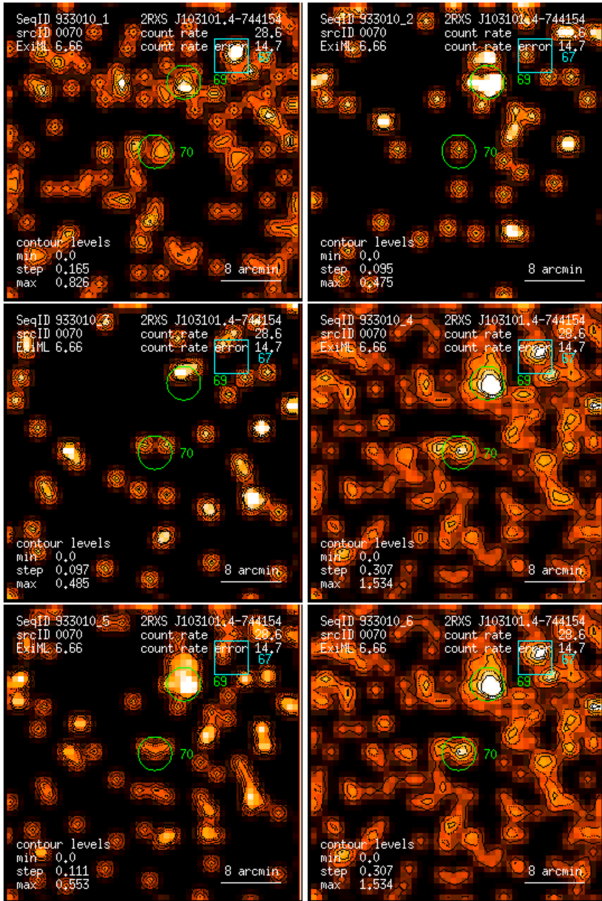
Figure 70: RASS 933010: detection 0070: band rate images, Gaussian filter: (1) PSPC channels 11 – 41, (2) 52 – 90, (3) 91 – 201, (4) 11 – 235, (5) 52 – 201, (6) 11 – 201. Broad band rates in counts/ks. Band rate contour levels in counts/ks/arcmin 2 .
