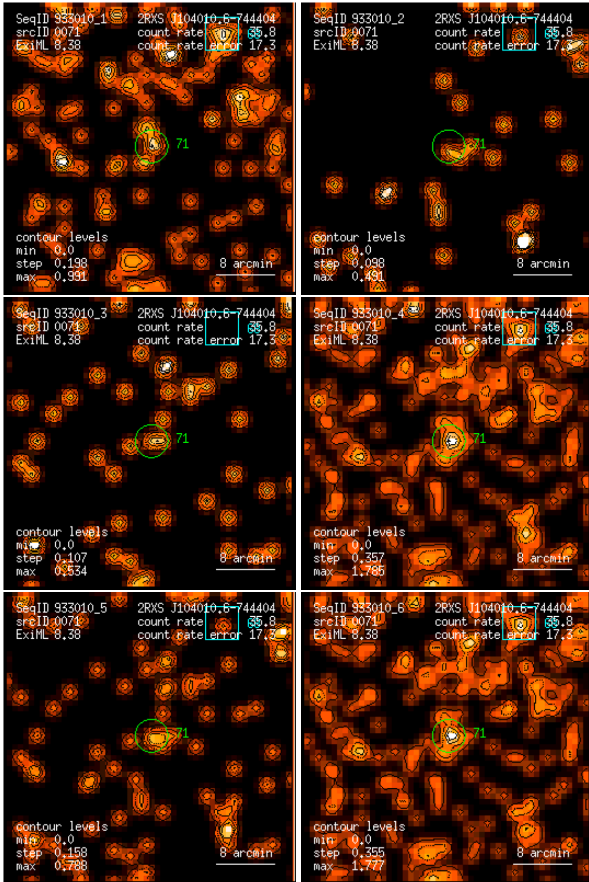
Figure 71: RASS 933010: detection 0071: band rate images, Gaussian filter: (1) PSPC channels 11 – 41, (2) 52 – 90, (3) 91 – 201, (4) 11 – 235, (5) 52 – 201, (6) 11 – 201. Broad band rates in counts/ks. Band rate contour levels in counts/ks/arcmin 2 .
