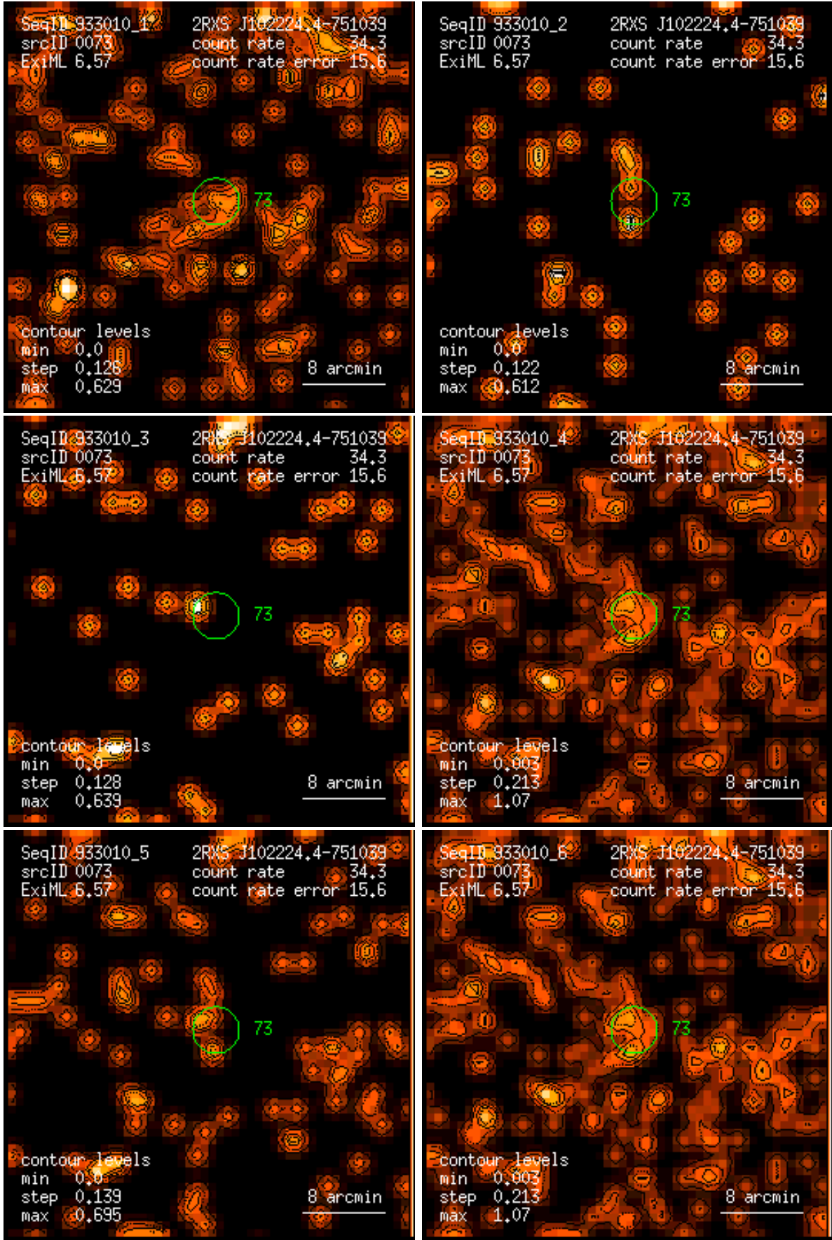
Figure 73: RASS 933010: detection 0073: band rate images, Gaussian filter: (1) PSPC channels 11 – 41, (2) 52 – 90, (3) 91 – 201, (4) 11 – 235, (5) 52 – 201, (6) 11 – 201. Broad band rates in counts/ks. Band rate contour levels in counts/ks/arcmin 2 .
