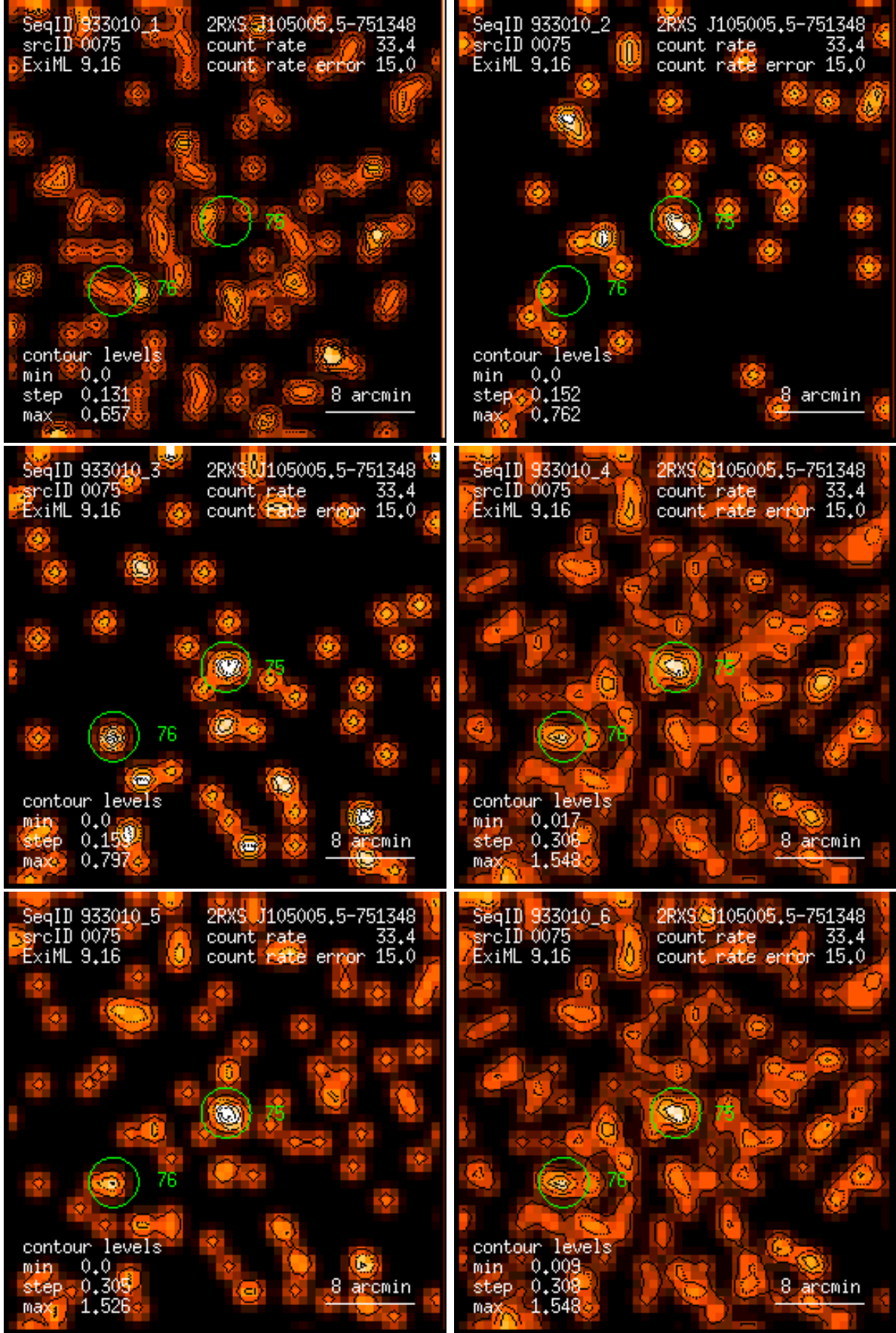
Figure 75: RASS 933010: detection 0075: band rate images, Gaussian filter: (1) PSPC channels 11 – 41, (2) 52 – 90, (3) 91 – 201, (4) 11 – 235, (5) 52 – 201, (6) 11 – 201. Broad band rates in counts/ks. Band rate contour levels in counts/ks/arcmin 2 .
