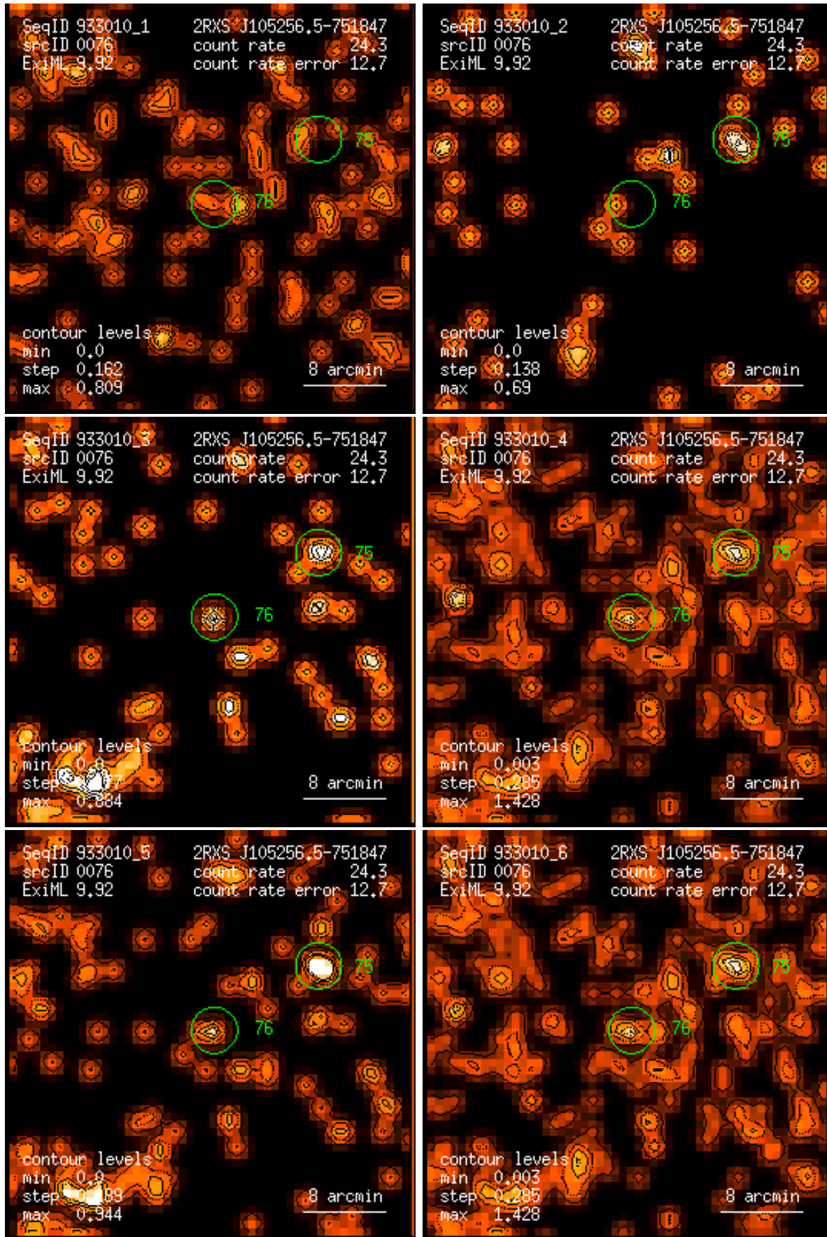
Figure 76: RASS 933010: detection 0076: band rate images, Gaussian filter: (1) PSPC channels 11 – 41, (2) 52 – 90, (3) 91 – 201, (4) 11 – 235, (5) 52 – 201, (6) 11 – 201. Broad band rates in counts/ks. Band rate contour levels in counts/ks/arcmin 2 .
