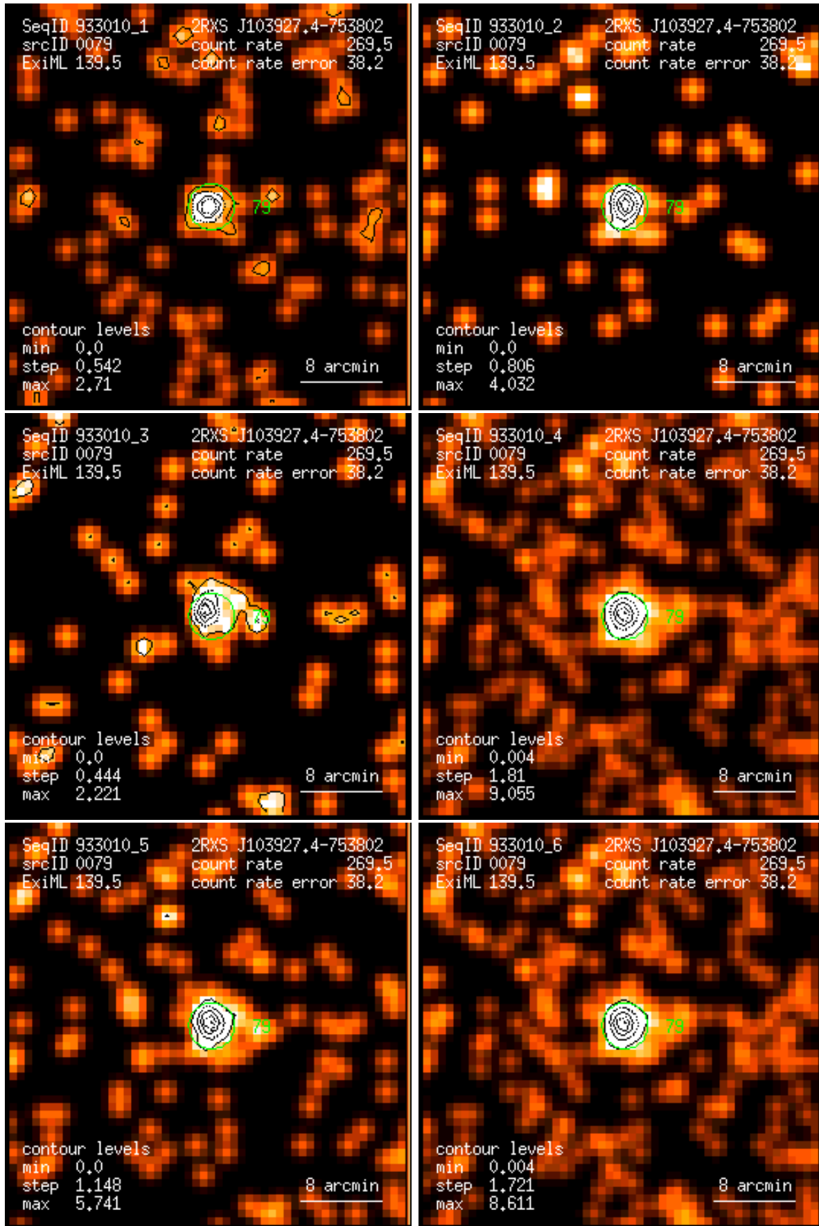
Figure 79: RASS 933010: detection 0079: band rate images, Gaussian filter: (1) PSPC channels 11 – 41, (2) 52 – 90, (3) 91 – 201, (4) 11 – 235, (5) 52 – 201, (6) 11 – 201. Broad band rates in counts/ks. Band rate contour levels in counts/ks/arcmin 2 .
