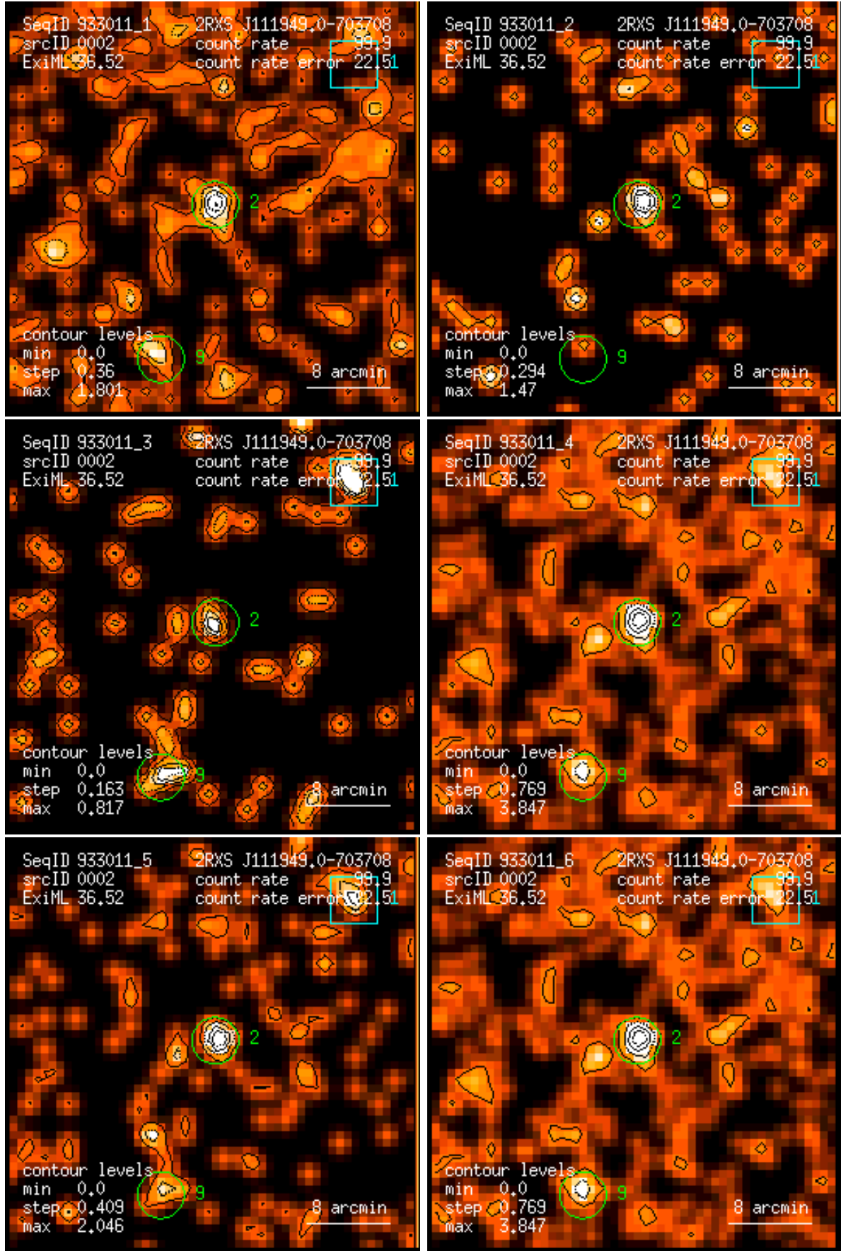
Figure 2: RASS 933011: detection 0002: band rate images, Gaussian filter: (1) PSPC channels 11 – 41, (2) 52 – 90, (3) 91 – 201, (4) 11 – 235, (5) 52 – 201, (6) 11 – 201. Broad band rates in counts/ks. Band rate contour levels in counts/ks/arcmin 2 .
