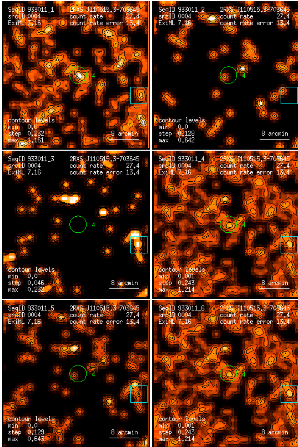
Figure 4: RASS 933011: detection 0004: band rate images, Gaussian filter: (1) PSPC channels 11 – 41, (2) 52 – 90, (3) 91 – 201, (4) 11 – 235, (5) 52 – 201, (6) 11 – 201. Broad band rates in counts/ks. Band rate contour levels in counts/ks/arcmin 2 .
