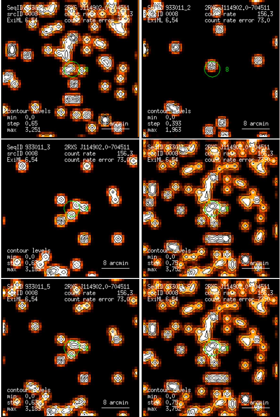
Figure 8: RASS 933011: detection 0008: band rate images, Gaussian filter: (1) PSPC channels 11 – 41, (2) 52 – 90, (3) 91 – 201, (4) 11 – 235, (5) 52 – 201, (6) 11 – 201. Broad band rates in counts/ks. Band rate contour levels in counts/ks/arcmin 2 .
