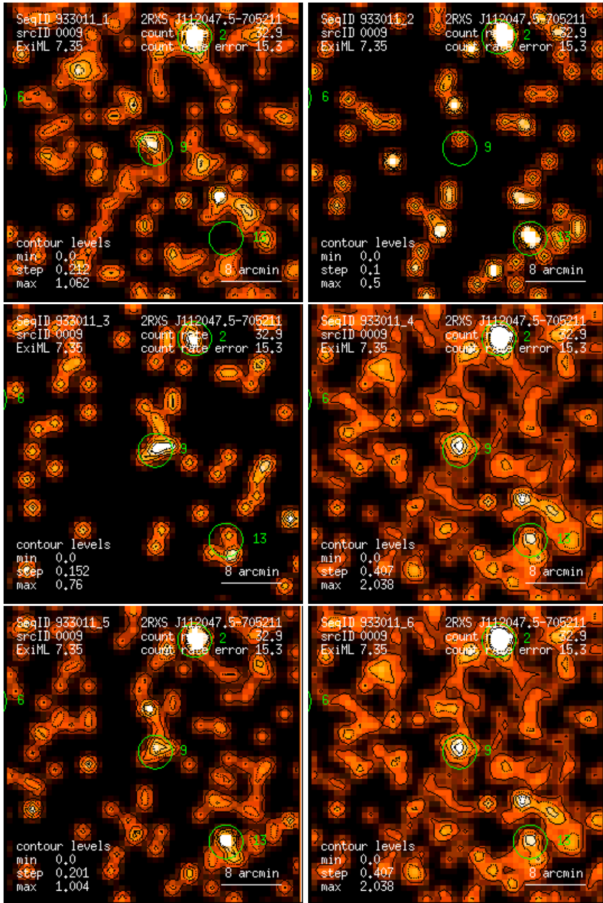
Figure 9: RASS 933011: detection 0009: band rate images, Gaussian filter: (1) PSPC channels 11 – 41, (2) 52 – 90, (3) 91 – 201, (4) 11 – 235, (5) 52 – 201, (6) 11 – 201. Broad band rates in counts/ks. Band rate contour levels in counts/ks/arcmin 2 .
