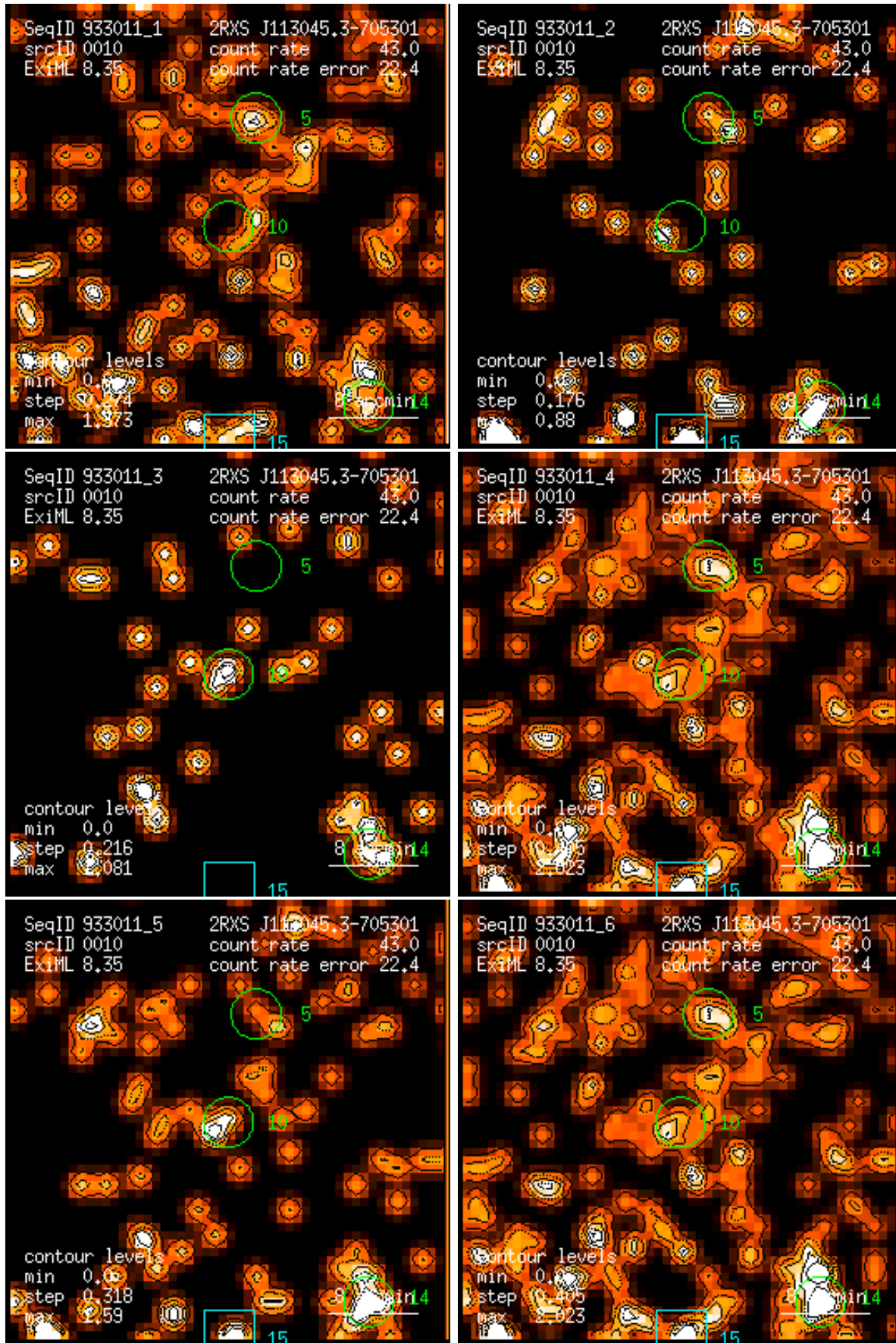
Figure 10: RASS 933011: detection 0010: band rate images, Gaussian filter: (1) PSPC channels 11 – 41, (2) 52 – 90, (3) 91 – 201, (4) 11 – 235, (5) 52 – 201, (6) 11 – 201. Broad band rates in counts/ks. Band rate contour levels in counts/ks/arcmin 2 .
