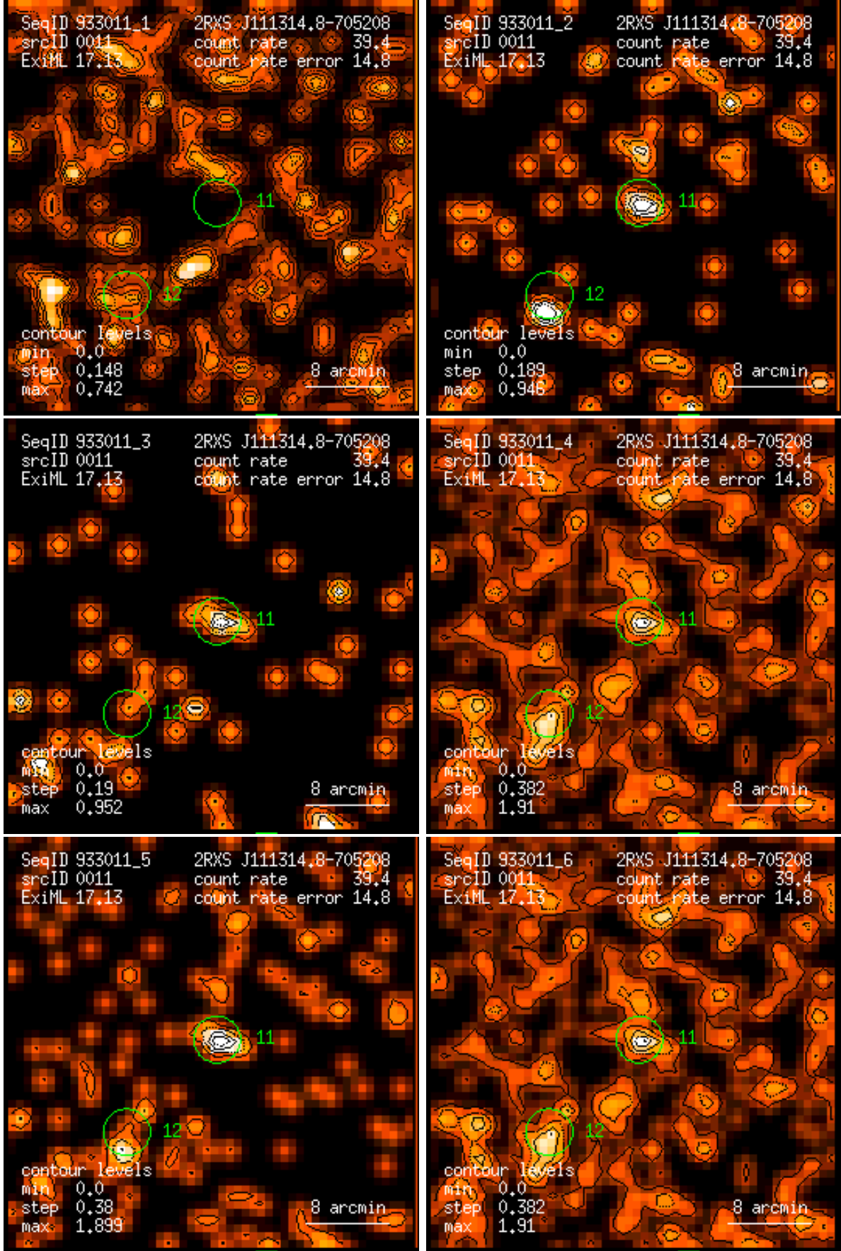
Figure 11: RASS 933011: detection 0011: band rate images, Gaussian filter: (1) PSPC channels 11 – 41, (2) 52 – 90, (3) 91 – 201, (4) 11 – 235, (5) 52 – 201, (6) 11 – 201. Broad band rates in counts/ks. Band rate contour levels in counts/ks/arcmin 2 .
