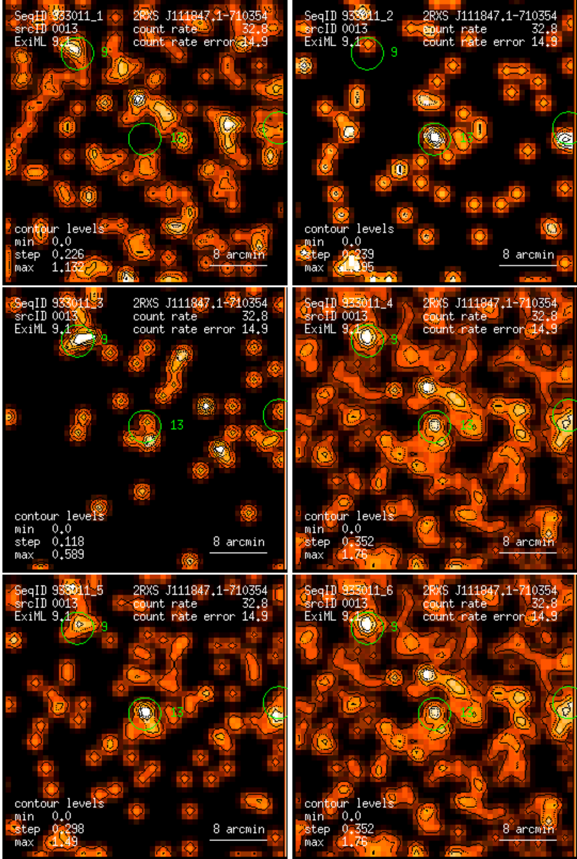
Figure 13: RASS 933011: detection 0013: band rate images, Gaussian filter: (1) PSPC channels 11 – 41, (2) 52 – 90, (3) 91 – 201, (4) 11 – 235, (5) 52 – 201, (6) 11 – 201. Broad band rates in counts/ks. Band rate contour levels in counts/ks/arcmin 2 .
