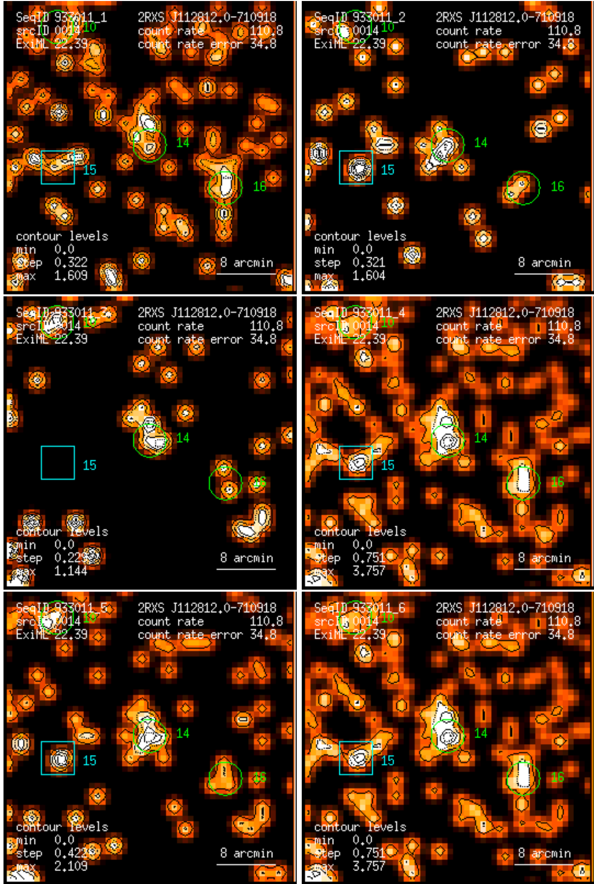
Figure 14: RASS 933011: detection 0014: band rate images, Gaussian filter: (1) PSPC channels 11 – 41, (2) 52 – 90, (3) 91 – 201, (4) 11 – 235, (5) 52 – 201, (6) 11 – 201. Broad band rates in counts/ks. Band rate contour levels in counts/ks/arcmin 2 .
