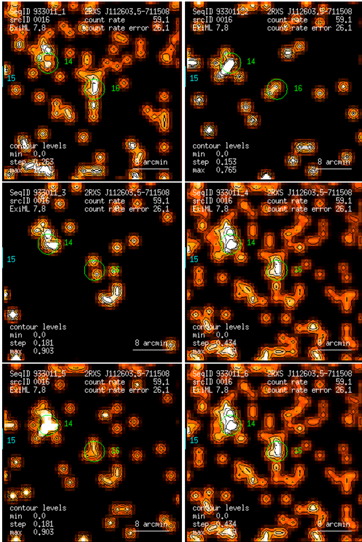
Figure 16: RASS 933011: detection 0016: band rate images, Gaussian filter: (1) PSPC channels 11 – 41, (2) 52 – 90, (3) 91 – 201, (4) 11 – 235, (5) 52 – 201, (6) 11 – 201. Broad band rates in counts/ks. Band rate contour levels in counts/ks/arcmin 2 .
