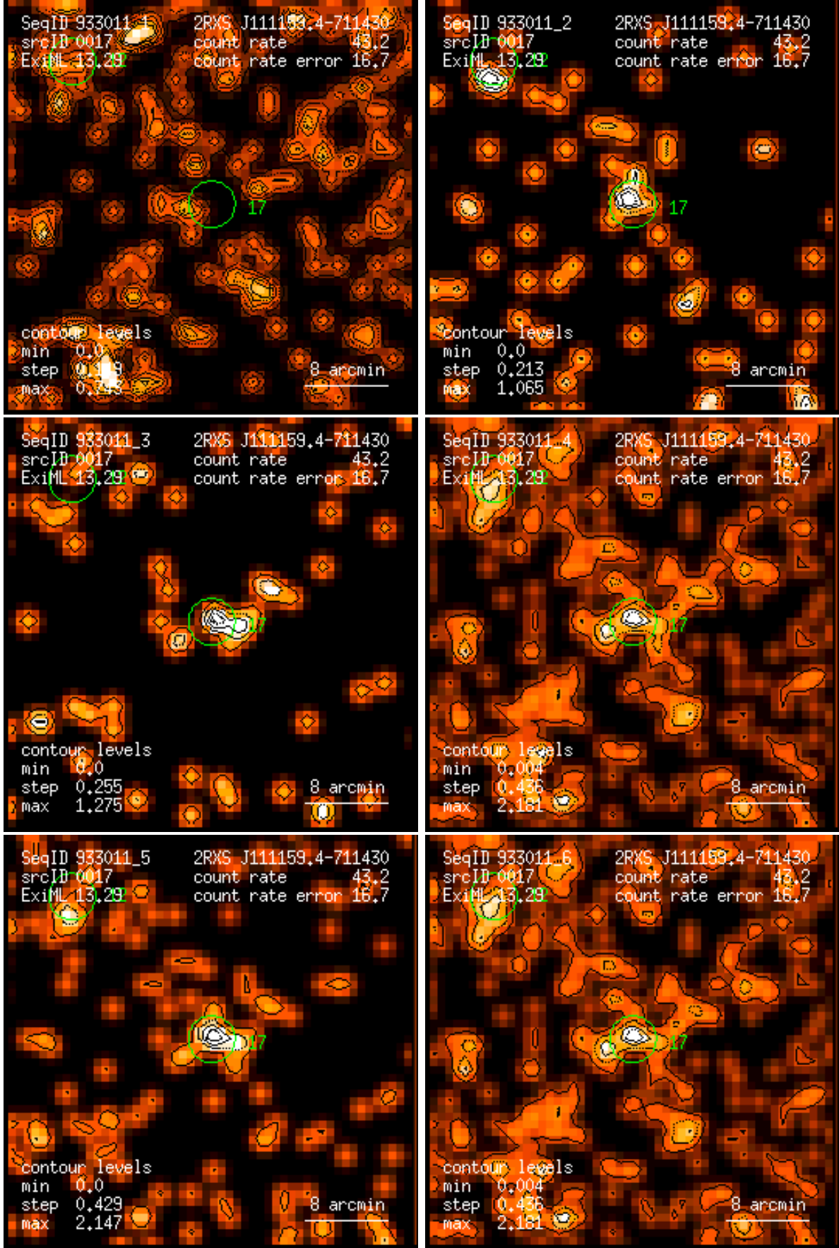
Figure 17: RASS 933011: detection 0017: band rate images, Gaussian filter: (1) PSPC channels 11 – 41, (2) 52 – 90, (3) 91 – 201, (4) 11 – 235, (5) 52 – 201, (6) 11 – 201. Broad band rates in counts/ks. Band rate contour levels in counts/ks/arcmin 2 .
