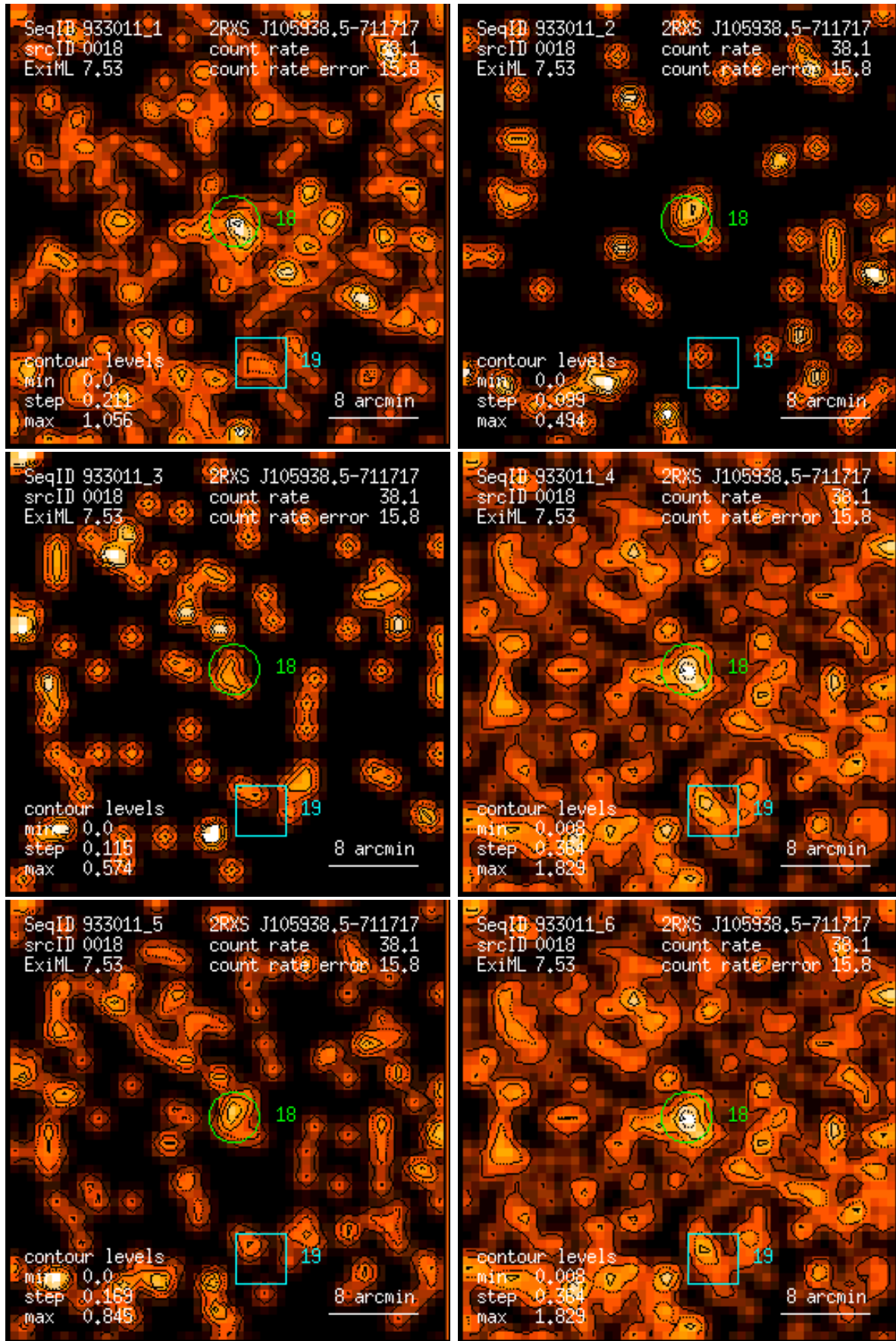
Figure 18: RASS 933011: detection 0018: band rate images, Gaussian filter: (1) PSPC channels 11 – 41, (2) 52 – 90, (3) 91 – 201, (4) 11 – 235, (5) 52 – 201, (6) 11 – 201. Broad band rates in counts/ks. Band rate contour levels in counts/ks/arcmin 2 .
