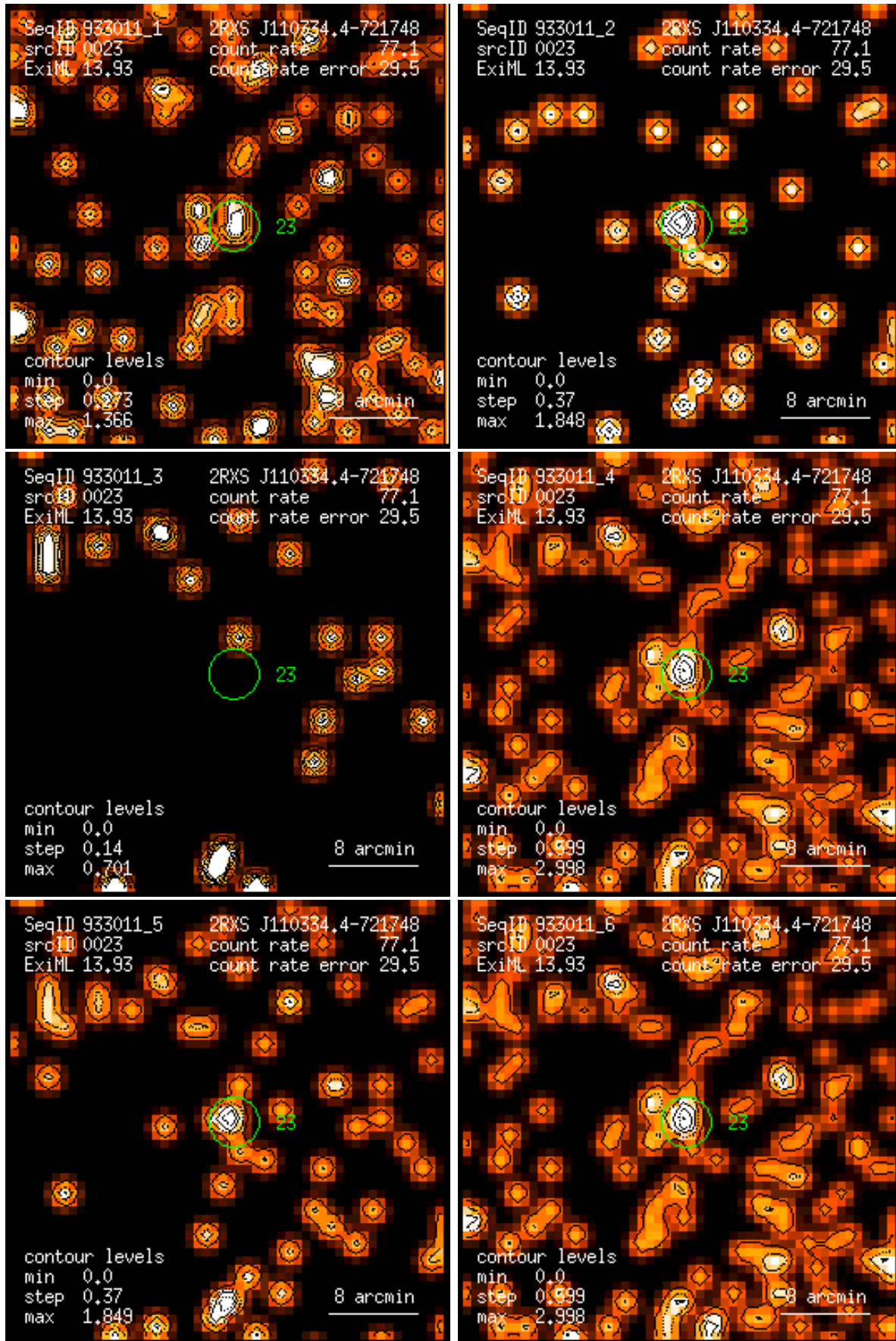
Figure 23: RASS 933011: detection 0023: band rate images, Gaussian filter: (1) PSPC channels 11 – 41, (2) 52 – 90, (3) 91 – 201, (4) 11 – 235, (5) 52 – 201, (6) 11 – 201. Broad band rates in counts/ks. Band rate contour levels in counts/ks/arcmin 2 .
