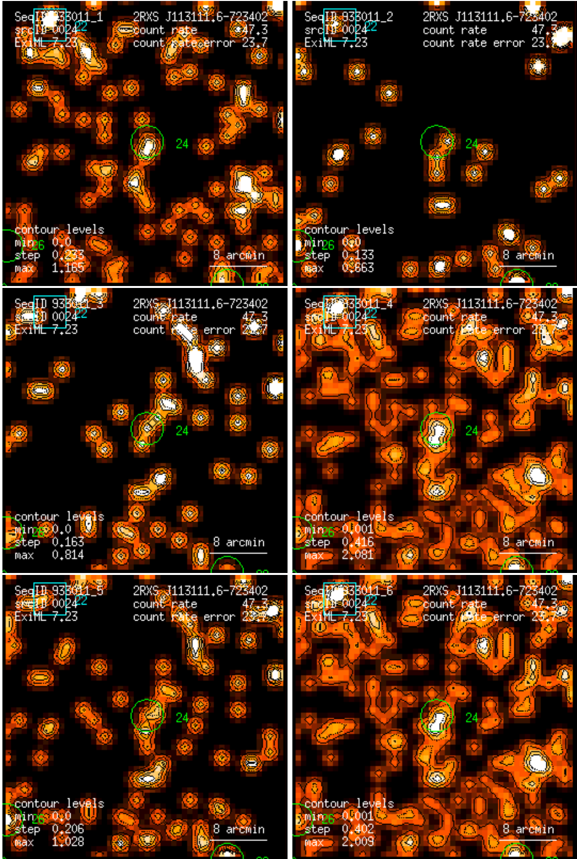
Figure 24: RASS 933011: detection 0024: band rate images, Gaussian filter: (1) PSPC channels 11 – 41, (2) 52 – 90, (3) 91 – 201, (4) 11 – 235, (5) 52 – 201, (6) 11 – 201. Broad band rates in counts/ks. Band rate contour levels in counts/ks/arcmin 2 .
