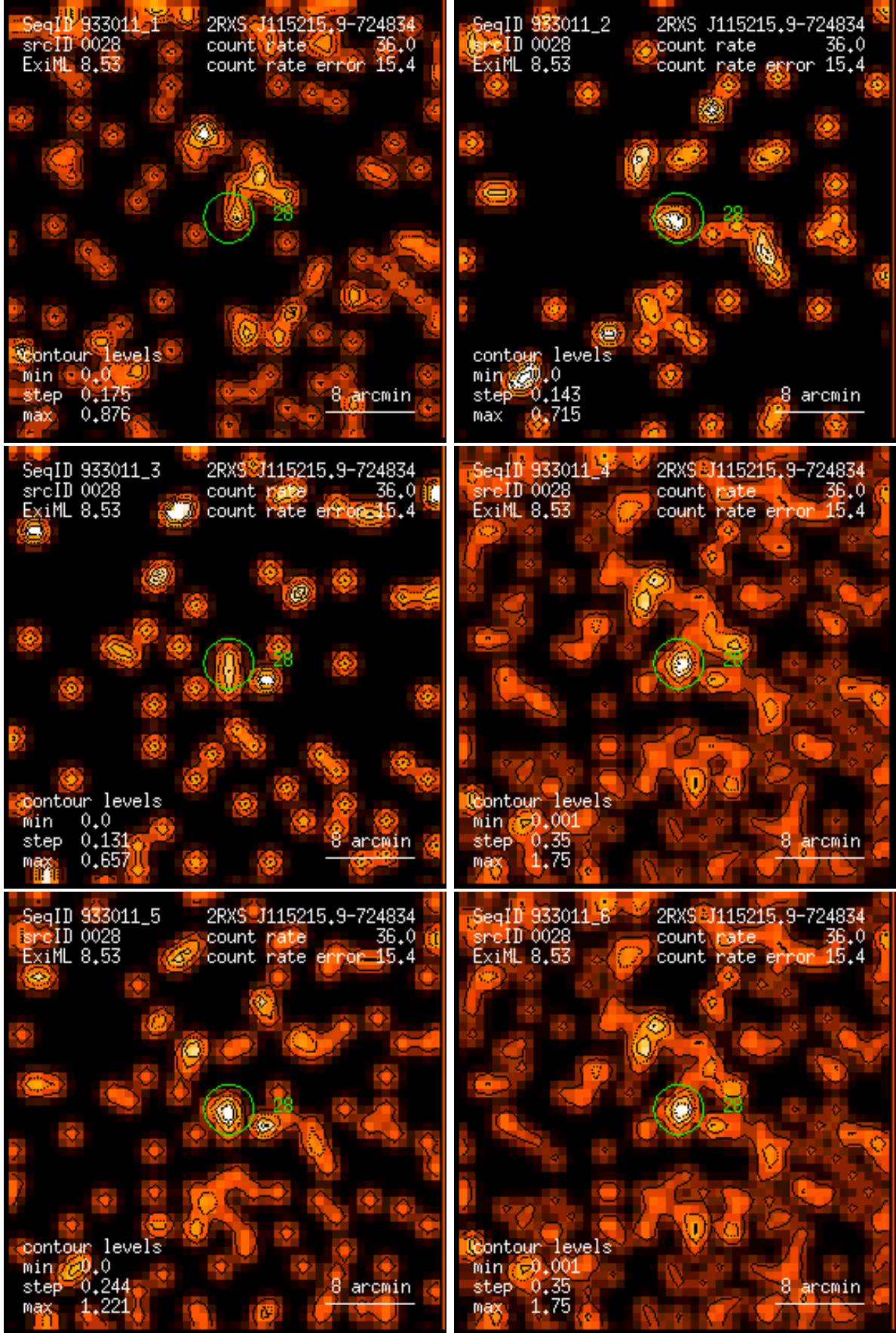
Figure 28: RASS 933011: detection 0028: band rate images, Gaussian filter: (1) PSPC channels 11 – 41, (2) 52 – 90, (3) 91 – 201, (4) 11 – 235, (5) 52 – 201, (6) 11 – 201. Broad band rates in counts/ks. Band rate contour levels in counts/ks/arcmin 2 .
