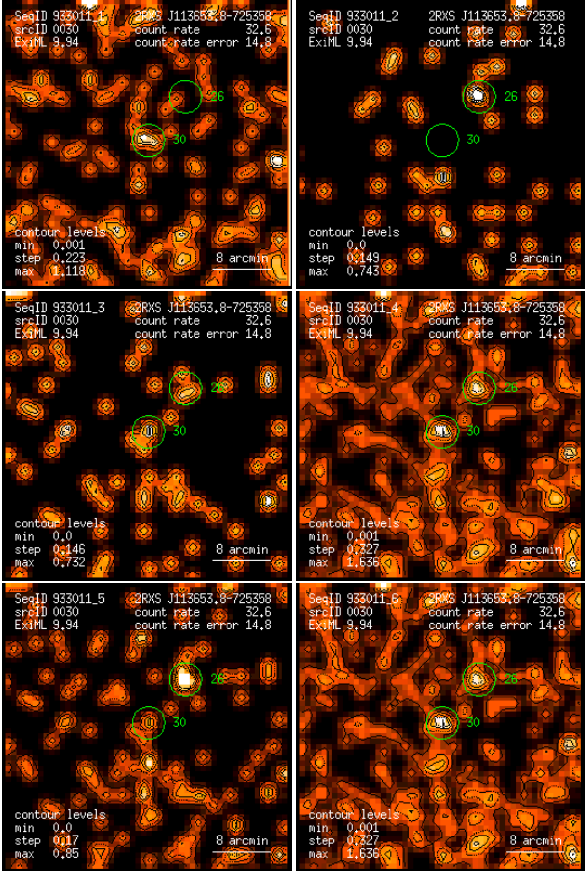
Figure 30: RASS 933011: detection 0030: band rate images, Gaussian filter: (1) PSPC channels 11 – 41, (2) 52 – 90, (3) 91 – 201, (4) 11 – 235, (5) 52 – 201, (6) 11 – 201. Broad band rates in counts/ks. Band rate contour levels in counts/ks/arcmin 2 .
