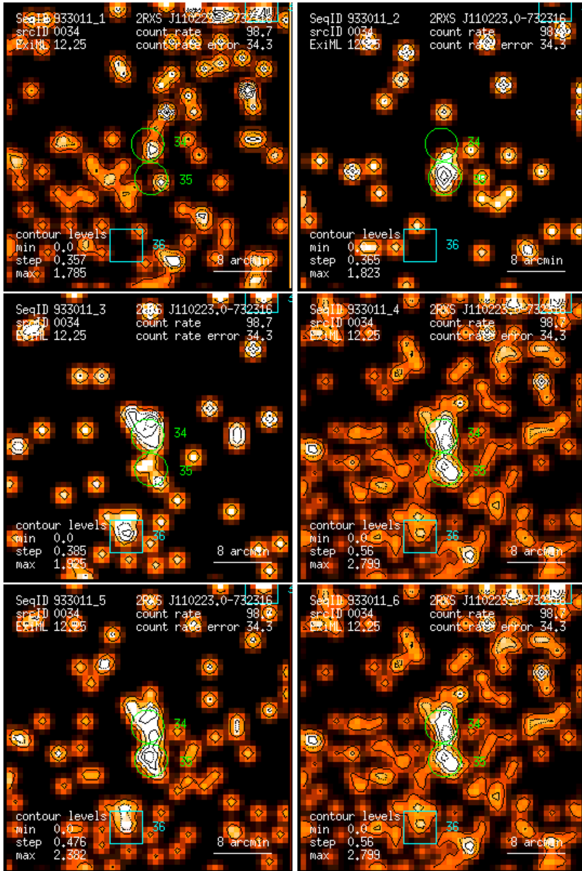
Figure 34: RASS 933011: detection 0034: band rate images, Gaussian filter: (1) PSPC channels 11 – 41, (2) 52 – 90, (3) 91 – 201, (4) 11 – 235, (5) 52 – 201, (6) 11 – 201. Broad band rates in counts/ks. Band rate contour levels in counts/ks/arcmin 2 .
