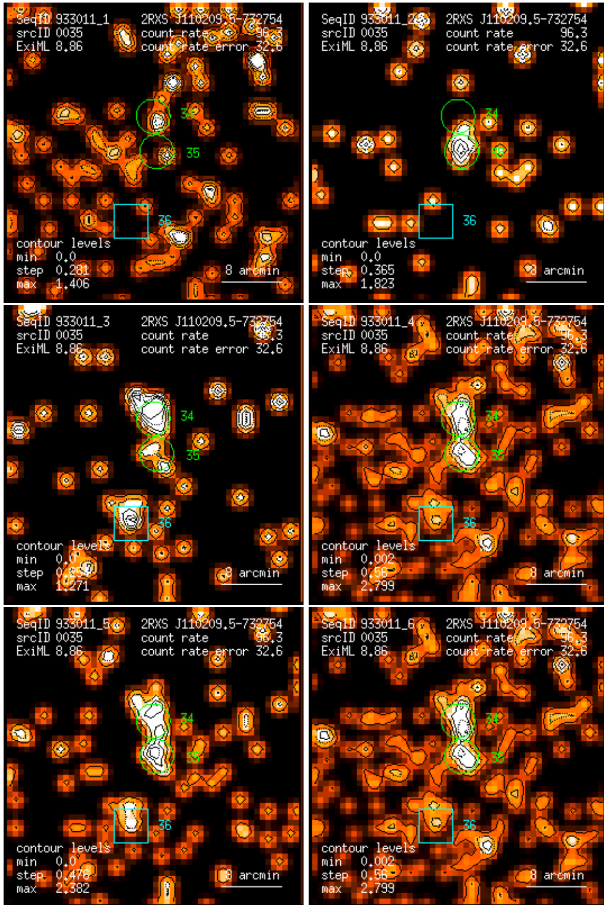
Figure 35: RASS 933011: detection 0035: band rate images, Gaussian filter: (1) PSPC channels 11 – 41, (2) 52 – 90, (3) 91 – 201, (4) 11 – 235, (5) 52 – 201, (6) 11 – 201. Broad band rates in counts/ks. Band rate contour levels in counts/ks/arcmin 2 .
