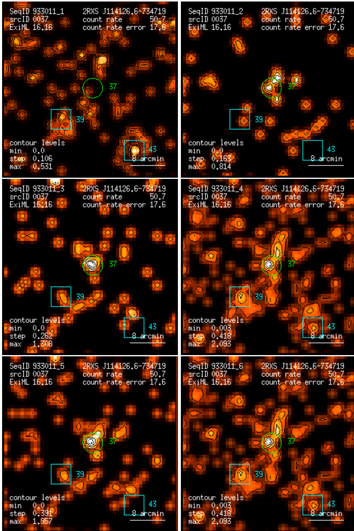
Figure 37: RASS 933011: detection 0037: band rate images, Gaussian filter: (1) PSPC channels 11 – 41, (2) 52 – 90, (3) 91 – 201, (4) 11 – 235, (5) 52 – 201, (6) 11 – 201. Broad band rates in counts/ks. Band rate contour levels in counts/ks/arcmin 2 .
