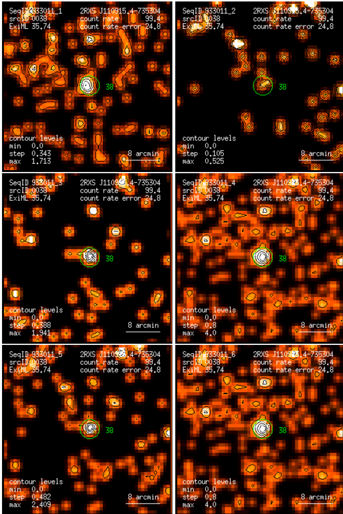
Figure 38: RASS 933011: detection 0038: band rate images, Gaussian filter: (1) PSPC channels 11 – 41, (2) 52 – 90, (3) 91 – 201, (4) 11 – 235, (5) 52 – 201, (6) 11 – 201. Broad band rates in counts/ks. Band rate contour levels in counts/ks/arcmin 2 .
