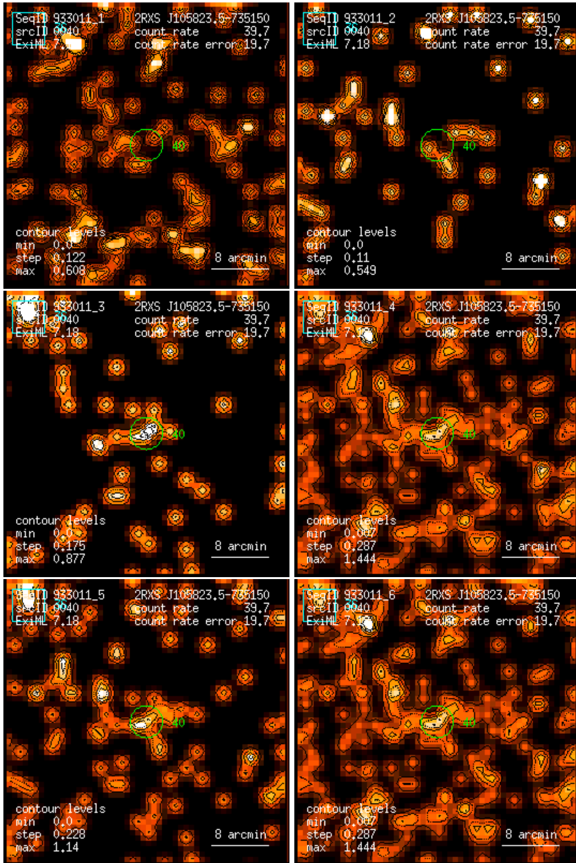
Figure 40: RASS 933011: detection 0040: band rate images, Gaussian filter: (1) PSPC channels 11 – 41, (2) 52 – 90, (3) 91 – 201, (4) 11 – 235, (5) 52 – 201, (6) 11 – 201. Broad band rates in counts/ks. Band rate contour levels in counts/ks/arcmin 2 .
