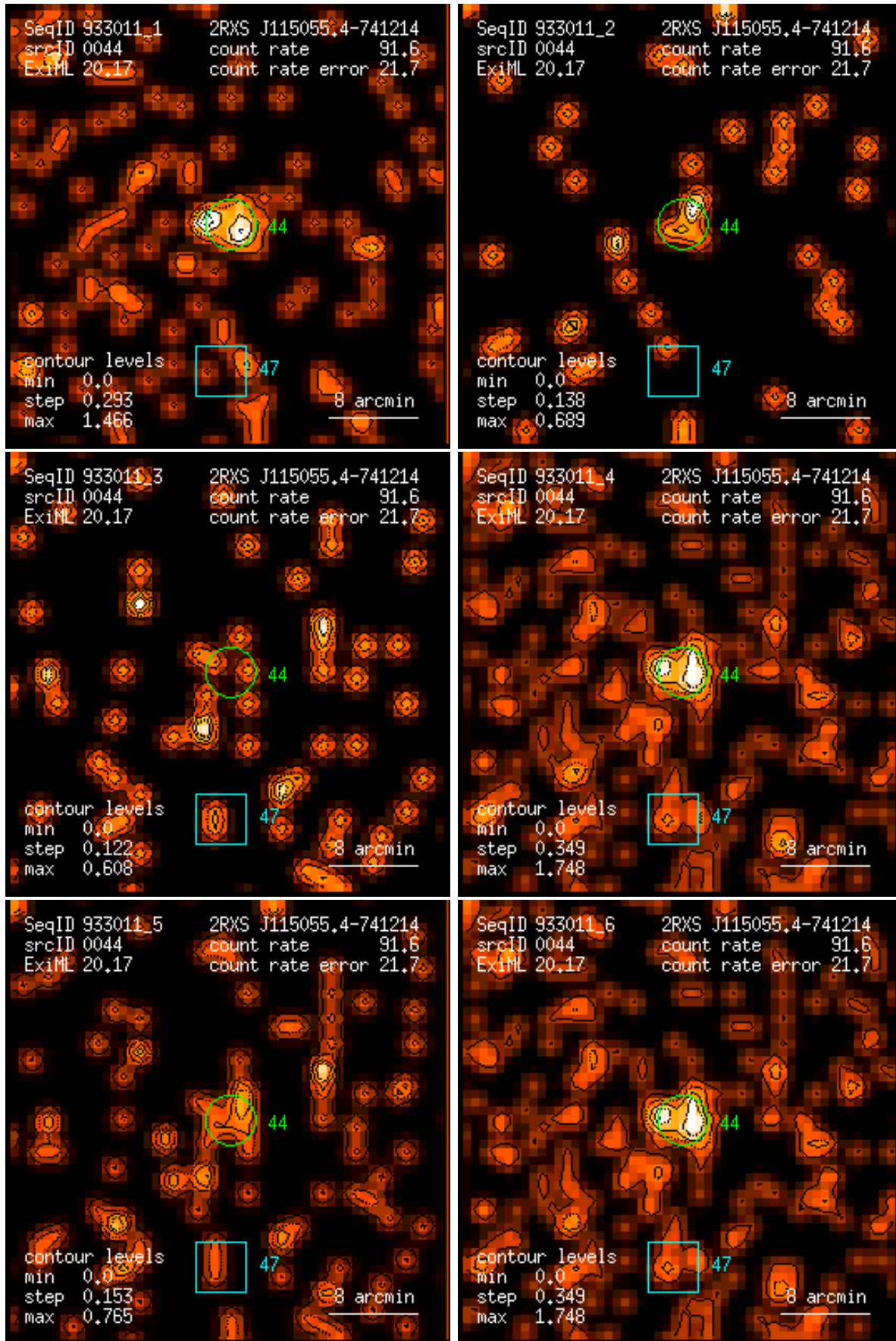
Figure 44: RASS 933011: detection 0044: band rate images, Gaussian filter: (1) PSPC channels 11 – 41, (2) 52 – 90, (3) 91 – 201, (4) 11 – 235, (5) 52 – 201, (6) 11 – 201. Broad band rates in counts/ks. Band rate contour levels in counts/ks/arcmin 2 .
