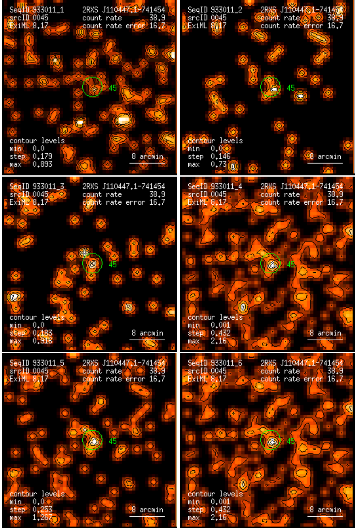
Figure 45: RASS 933011: detection 0045: band rate images, Gaussian filter: (1) PSPC channels 11 – 41, (2) 52 – 90, (3) 91 – 201, (4) 11 – 235, (5) 52 – 201, (6) 11 – 201. Broad band rates in counts/ks. Band rate contour levels in counts/ks/arcmin 2 .
