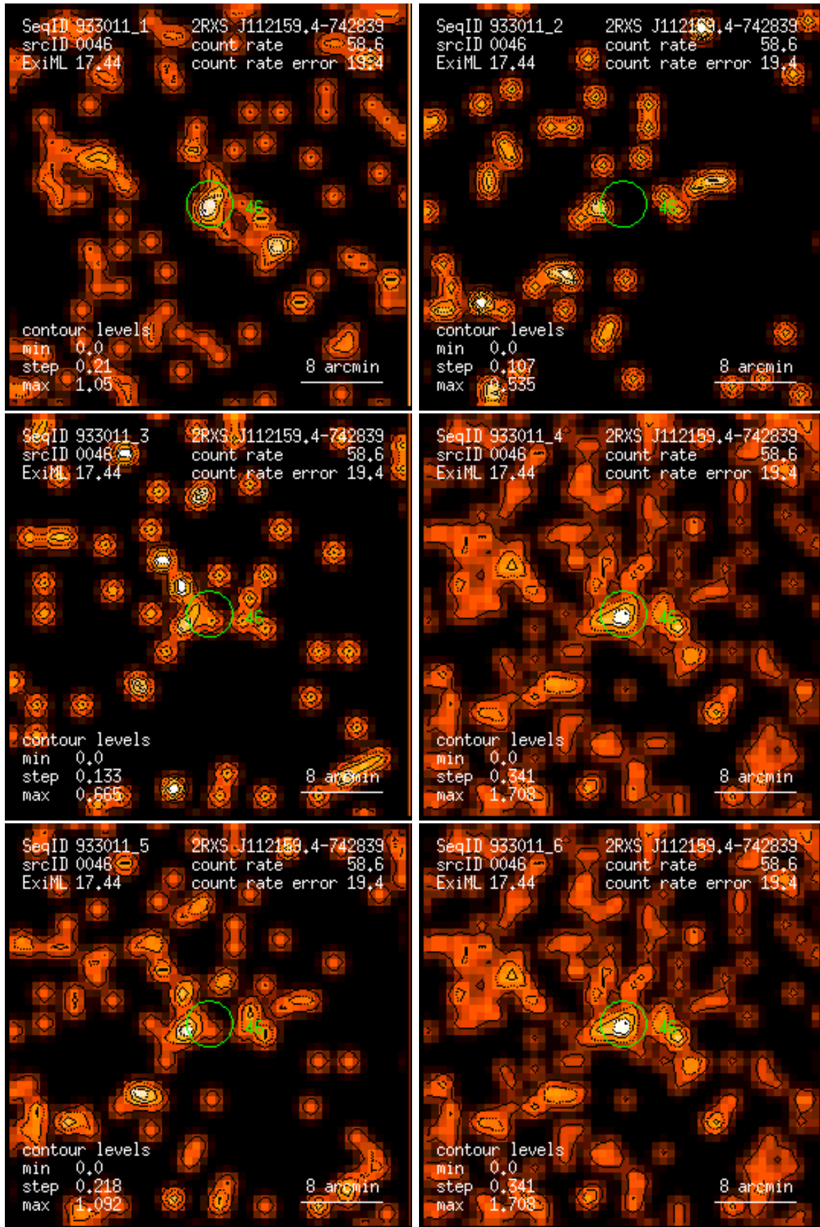
Figure 46: RASS 933011: detection 0046: band rate images, Gaussian filter: (1) PSPC channels 11 – 41, (2) 52 – 90, (3) 91 – 201, (4) 11 – 235, (5) 52 – 201, (6) 11 – 201. Broad band rates in counts/ks. Band rate contour levels in counts/ks/arcmin 2 .
