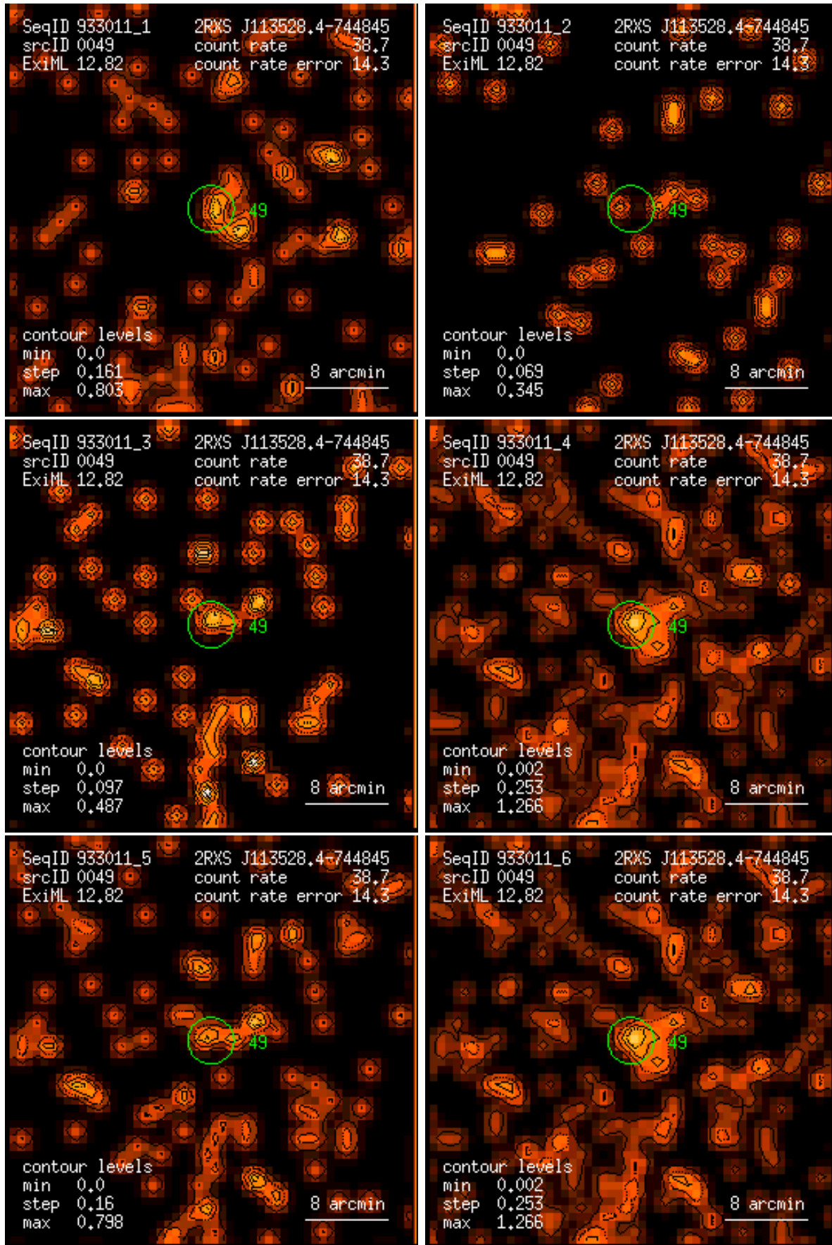
Figure 49: RASS 933011: detection 0049: band rate images, Gaussian filter: (1) PSPC channels 11 – 41, (2) 52 – 90, (3) 91 – 201, (4) 11 – 235, (5) 52 – 201, (6) 11 – 201. Broad band rates in counts/ks. Band rate contour levels in counts/ks/arcmin 2 .
