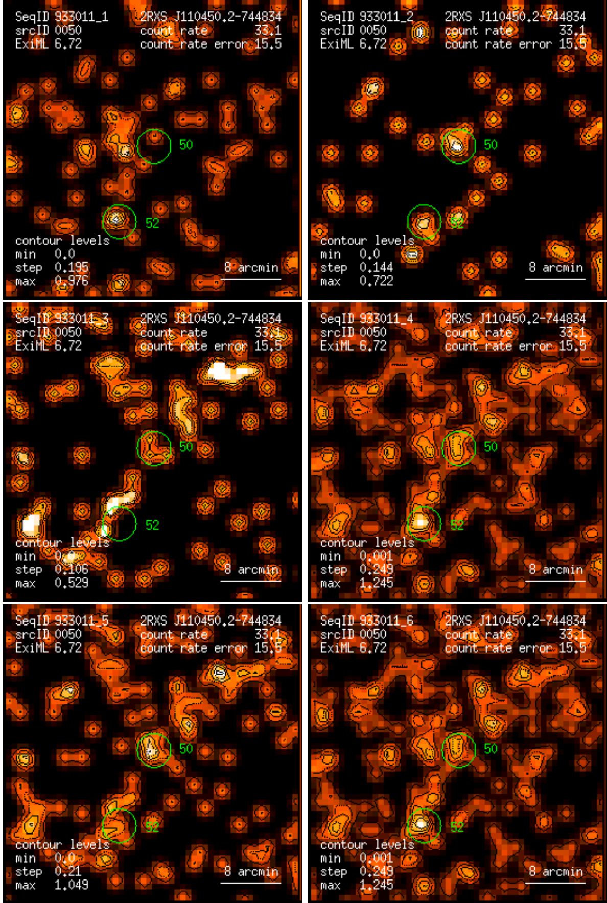
Figure 50: RASS 933011: detection 0050: band rate images, Gaussian filter: (1) PSPC channels 11 – 41, (2) 52 – 90, (3) 91 – 201, (4) 11 – 235, (5) 52 – 201, (6) 11 – 201. Broad band rates in counts/ks. Band rate contour levels in counts/ks/arcmin 2 .
