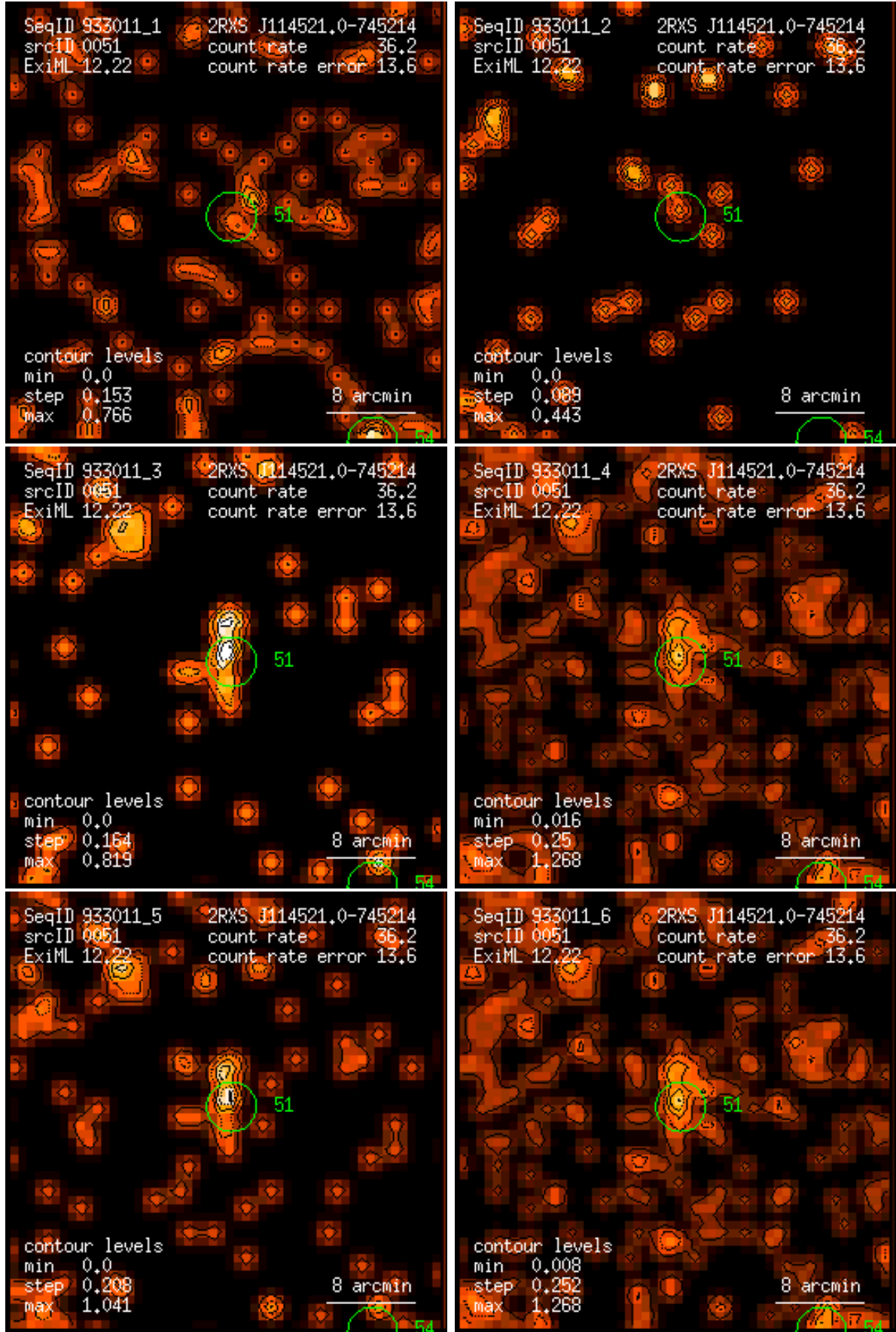
Figure 51: RASS 933011: detection 0051: band rate images, Gaussian filter: (1) PSPC channels 11 – 41, (2) 52 – 90, (3) 91 – 201, (4) 11 – 235, (5) 52 – 201, (6) 11 – 201. Broad band rates in counts/ks. Band rate contour levels in counts/ks/arcmin 2 .
