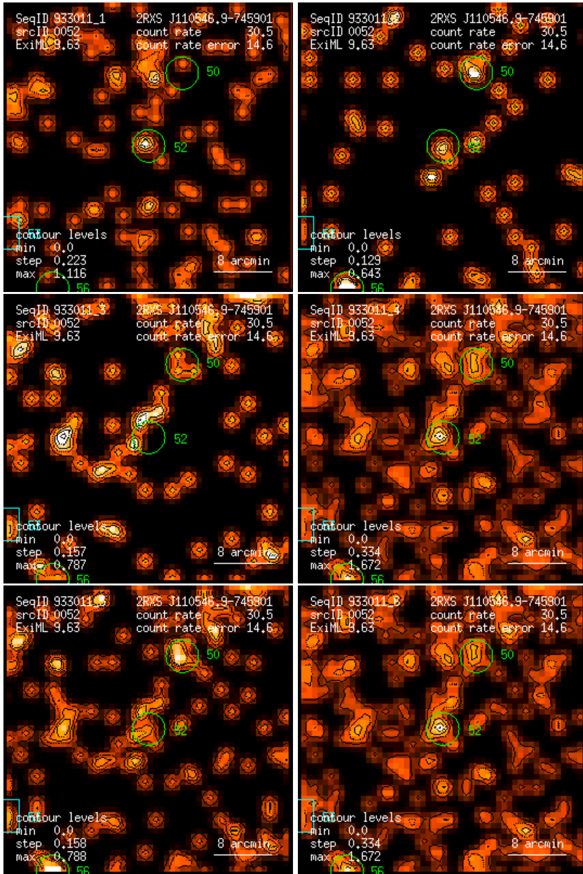
Figure 52: RASS 933011: detection 0052: band rate images, Gaussian filter: (1) PSPC channels 11 – 41, (2) 52 – 90, (3) 91 – 201, (4) 11 – 235, (5) 52 – 201, (6) 11 – 201. Broad band rates in counts/ks. Band rate contour levels in counts/ks/arcmin 2 .
