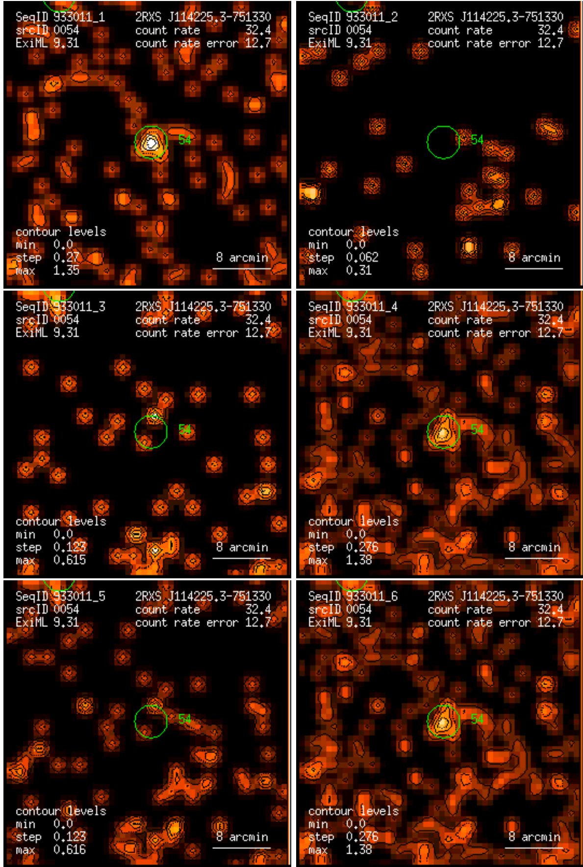
Figure 54: RASS 933011: detection 0054: band rate images, Gaussian filter: (1) PSPC channels 11 – 41, (2) 52 – 90, (3) 91 – 201, (4) 11 – 235, (5) 52 – 201, (6) 11 – 201. Broad band rates in counts/ks. Band rate contour levels in counts/ks/arcmin 2 .
