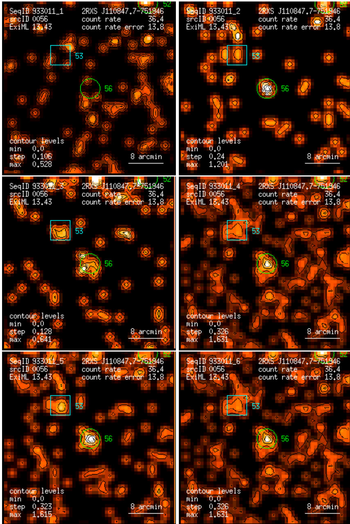
Figure 56: RASS 933011: detection 0056: band rate images, Gaussian filter: (1) PSPC channels 11 – 41, (2) 52 – 90, (3) 91 – 201, (4) 11 – 235, (5) 52 – 201, (6) 11 – 201. Broad band rates in counts/ks. Band rate contour levels in counts/ks/arcmin 2 .
