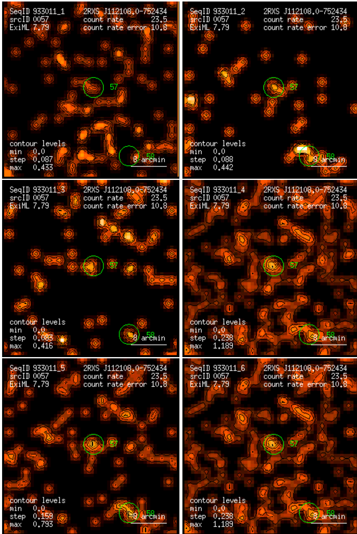
Figure 57: RASS 933011: detection 0057: band rate images, Gaussian filter: (1) PSPC channels 11 – 41, (2) 52 – 90, (3) 91 – 201, (4) 11 – 235, (5) 52 – 201, (6) 11 – 201. Broad band rates in counts/ks. Band rate contour levels in counts/ks/arcmin 2 .
