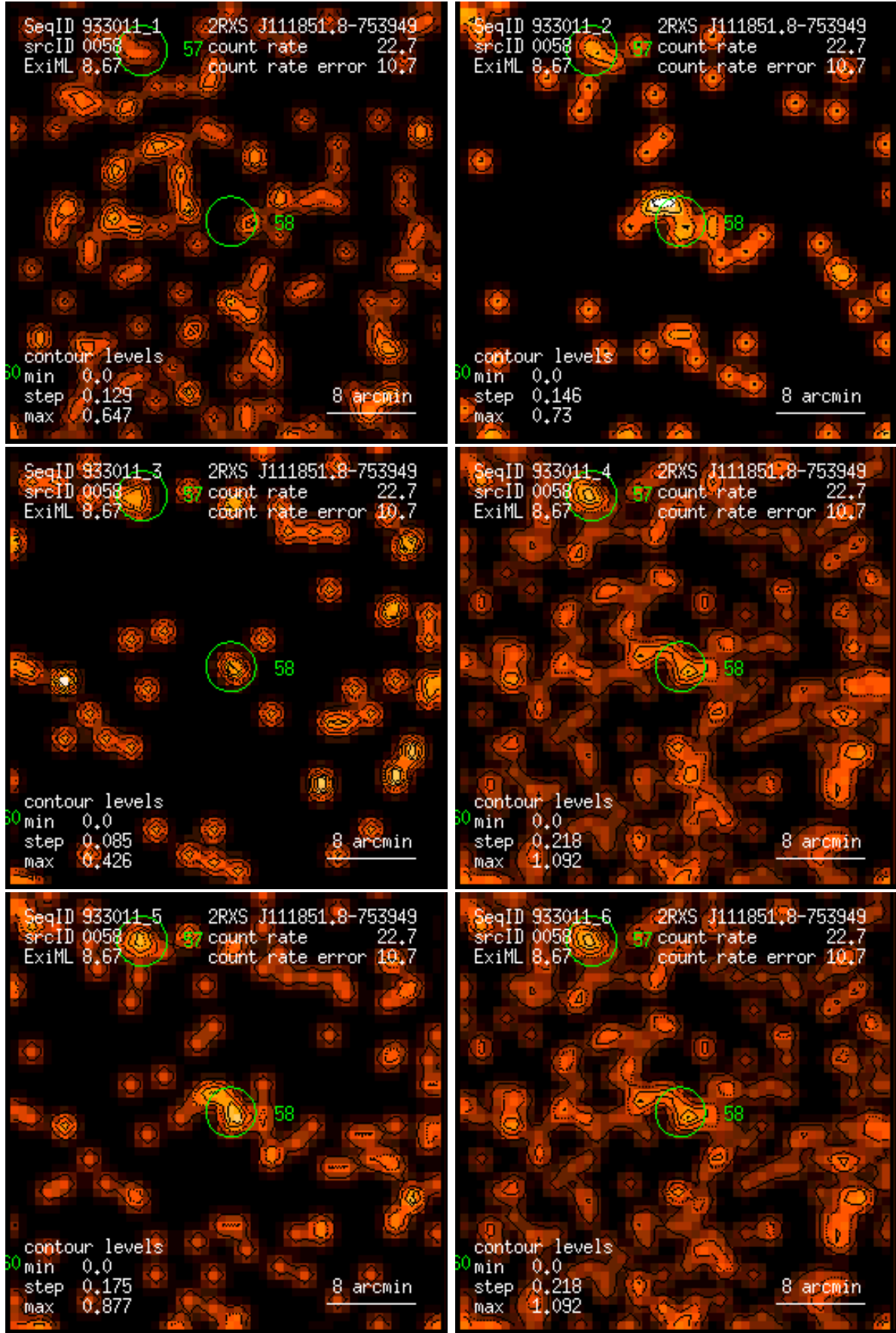
Figure 58: RASS 933011: detection 0058: band rate images, Gaussian filter: (1) PSPC channels 11 – 41, (2) 52 – 90, (3) 91 – 201, (4) 11 – 235, (5) 52 – 201, (6) 11 – 201. Broad band rates in counts/ks. Band rate contour levels in counts/ks/arcmin 2 .
