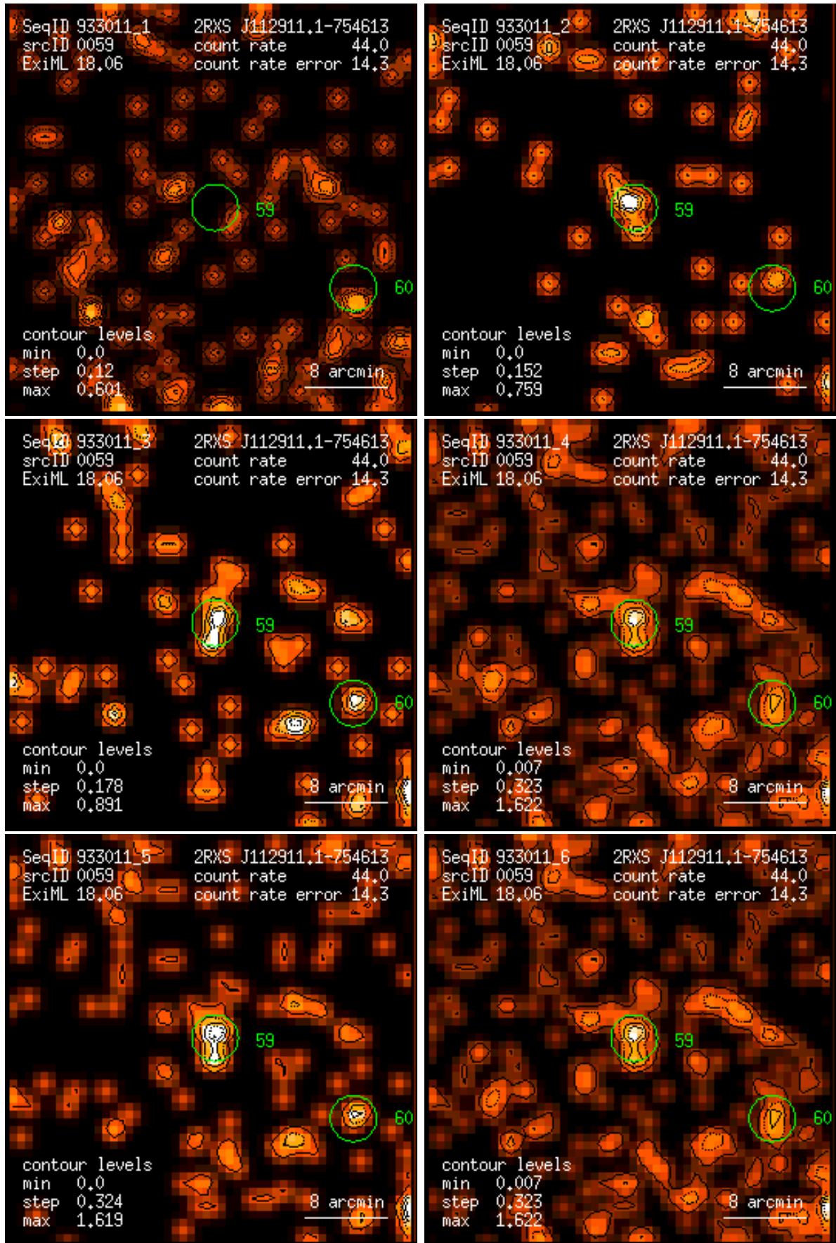
Figure 59: RASS 933011: detection 0059: band rate images, Gaussian filter: (1) PSPC channels 11 – 41, (2) 52 – 90, (3) 91 – 201, (4) 11 – 235, (5) 52 – 201, (6) 11 – 201. Broad band rates in counts/ks. Band rate contour levels in counts/ks/arcmin 2 .
