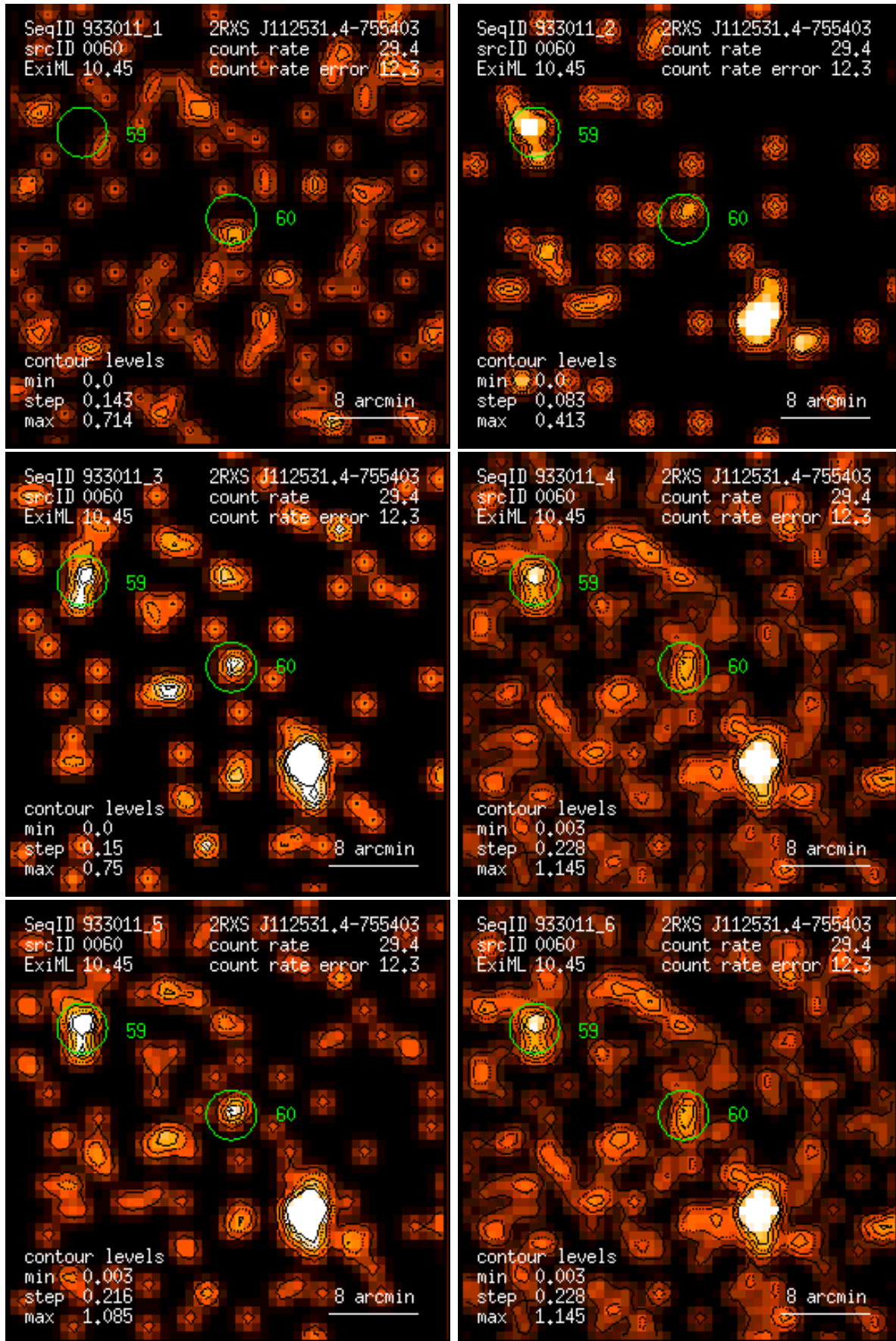
Figure 60: RASS 933011: detection 0060: band rate images, Gaussian filter: (1) PSPC channels 11 – 41, (2) 52 – 90, (3) 91 – 201, (4) 11 – 235, (5) 52 – 201, (6) 11 – 201. Broad band rates in counts/ks. Band rate contour levels in counts/ks/arcmin 2 .
