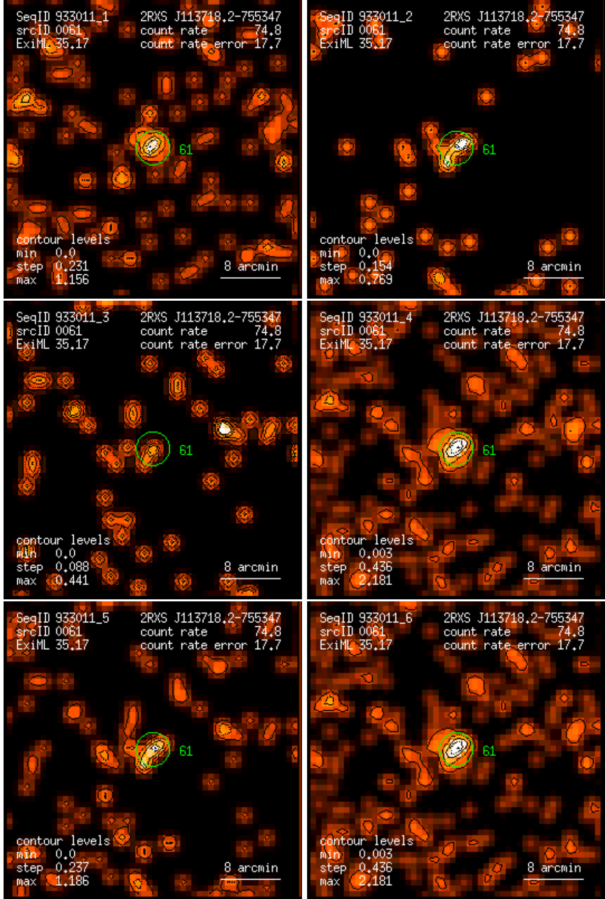
Figure 61: RASS 933011: detection 0061: band rate images, Gaussian filter: (1) PSPC channels 11 – 41, (2) 52 – 90, (3) 91 – 201, (4) 11 – 235, (5) 52 – 201, (6) 11 – 201. Broad band rates in counts/ks. Band rate contour levels in counts/ks/arcmin 2 .
